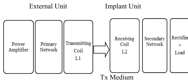
FIGURE 2. Inductive wireless power transmission network.
