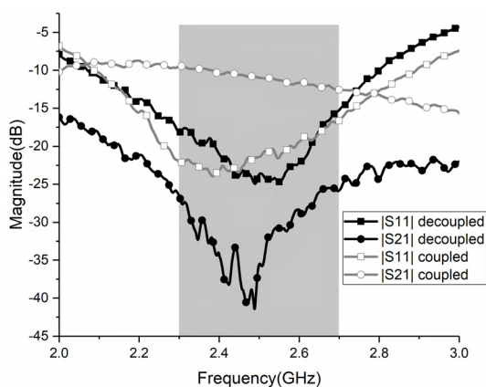
FIGURE 6. Measured S-parameters of the coupled and decoupled antennas.
