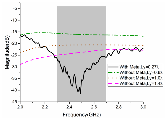
FIGURE 10. Simulated isolation of two bowtie antennas with different center to center spacing compared with the antennas with the metasurface superstrate.
