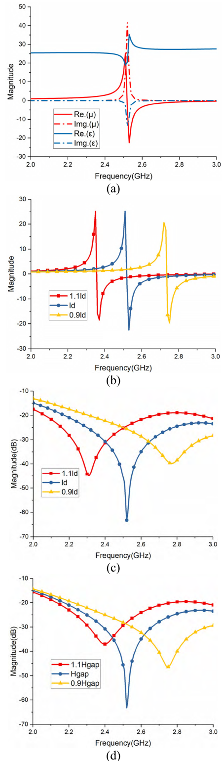
FIGURE 4. (a) Extracted permittivity and permeability of the metasurface using double layer cut wires as unit cell. (b) Extracted permeabilities with respect to different cut wire lengths. Decoupling frequency bands with respect to (c) different cut wire lengths and (d) different heights of the metasurface.
