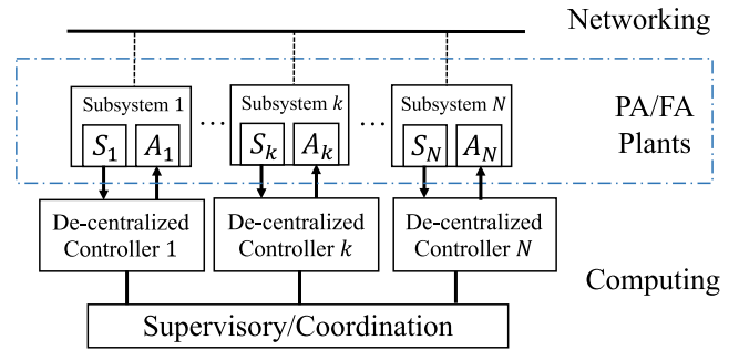
FIGURE 5. Structure of Decentralized Control.
