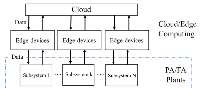
FIGURE 9. Structure of Hybrid Cloud and Edge Computing for I-IoT.
