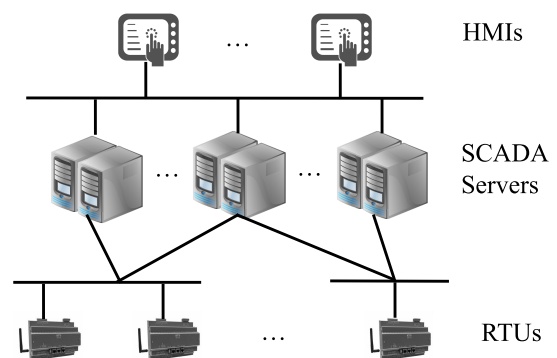
FIGURE 6. Simplified SCADA Architecture.
