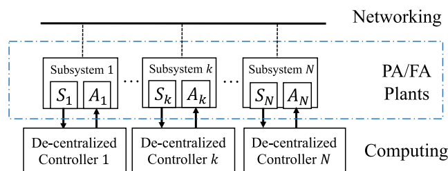
FIGURE 4. Structure of Centralized Control.
