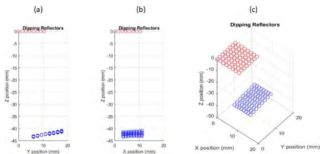
FIGURE 7. Example surface mapping results for the dipping reflectors projection algorithm (a) y - z mapping. (b) x - z mapping. (c) x-y-z surface mapping sample.
