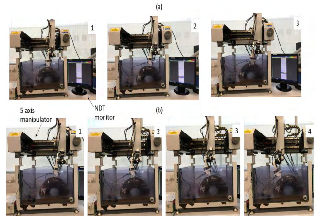
FIGURE 20. (a) Inspection example – cross section of the chain. (b) Inspection example – across the chain crown surface.
