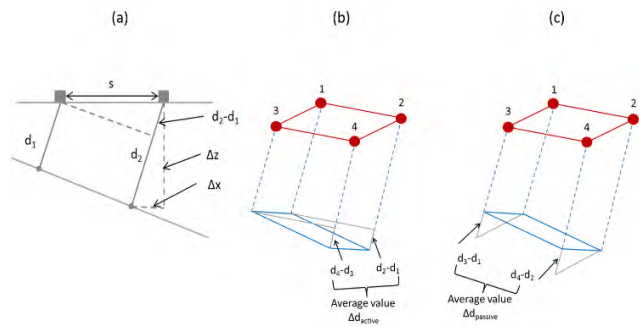
FIGURE 3. (a) Calculation of the shift in x and z from the transducer location using the difference in paths d_1 and d_2 . (b) and (c) Calculation of the average gradient in the active x and passive y array (blue).
