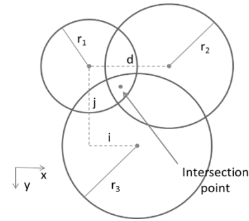
FIGURE 4. Calculation of the inspection point of three spheres array directions.
