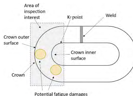
FIGURE 1. NDT inspection focused areas due to high stress which can cause fatigue cracking [20], [19].
