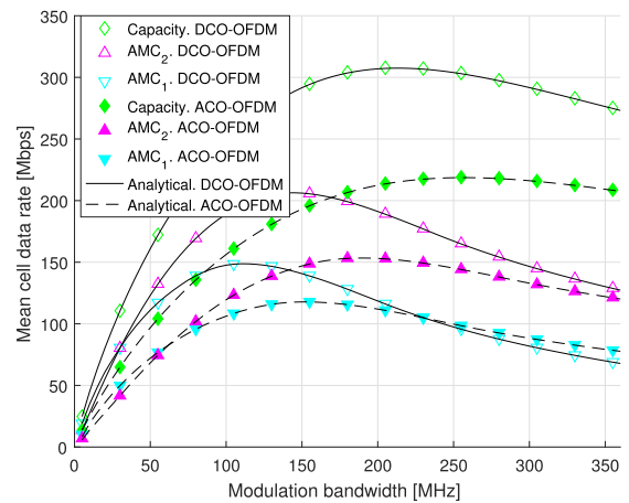
FIGURE 8. Average data rate s vs. bandwidth W at capacity, with AMC 1 and AMC 2 , at night ( E_{v,ab,vr} = 0 lux).
