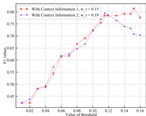
FIGURE 10. Best performances of SGNRI 1 (Word2Vec) and SGNRI 2 (Word2Vec).
