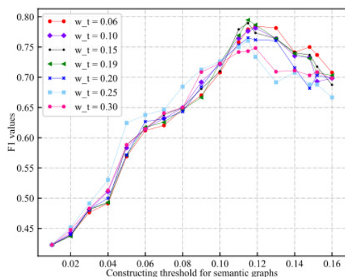
FIGURE 9. Performances of SGNRI 2 (Word2Vec).
