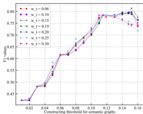
FIGURE 8. Performances of SGNRI 1 (Word2Vec).
