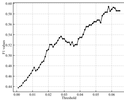
FIGURE 3. Results based on Word2Vec.
