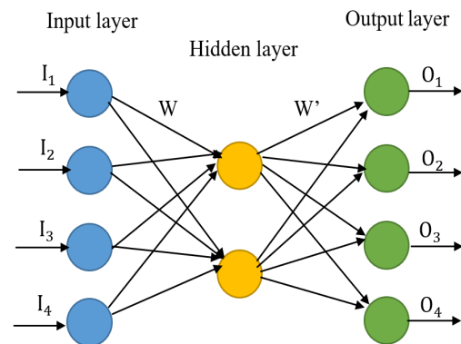
FIGURE 1. Autoencoder.
