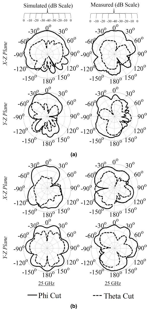
FIGURE 7. Radiation patterns of the MIMO antennas for smart 5G devices. (a): Polar patterns for antenna # 1 (b): Polar patterns for antenna # 5.
