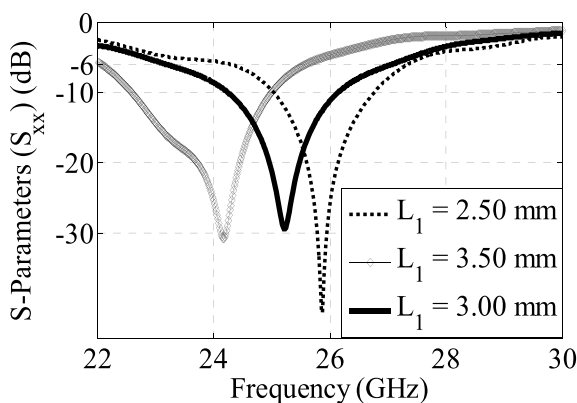
FIGURE 11. Effect of parameterization of the length 'L 1 ' on the S-Parameter (S xx ) of the proposed 5G MIMO antennas.
