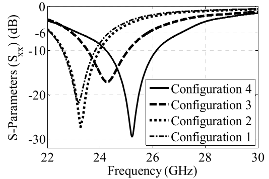
FIGURE 9. S-Parameter ( S_{xx} ) of the different configurations of the proposed 5G MIMO antennas.
