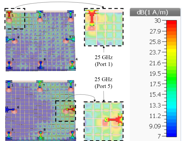
FIGURE 6. Surface current distributions of the 5G MIMO antennas.
