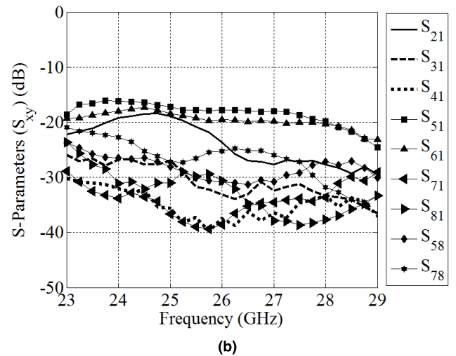
FIGURE 5. S_{XY} of the proposed 5G MIMO antennas. (a): Simulation results. (b): Measurement results.
