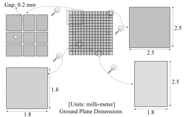
FIGURE 3. Detailed dimensions of the proposed MIMO antennas for smart 5G devices.
