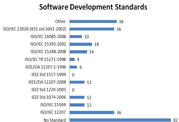
FIGURE 6. Frequency of adapted software development standard.
