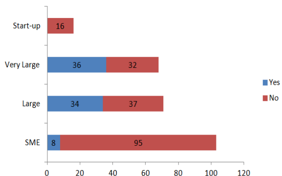
FIGURE 5. Frequency of defined measurement processes.
