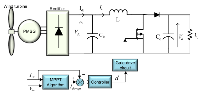
FIGURE 1. WECS configuration.
