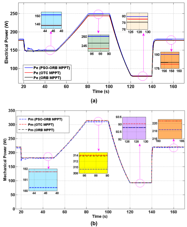
FIGURE 14. Performance comparison: Case 2 (a) electrical power (b) mechanical power.
