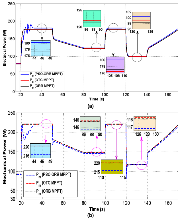
FIGURE 13. Performance comparison: Case 1 (a) electrical power (b) mechanical power.
