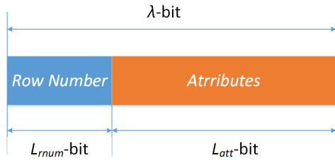
FIGURE 5. \lambda -bit length element of ACF with L_{rnum} -bit row number string and L_{att} -bit attribute string.
