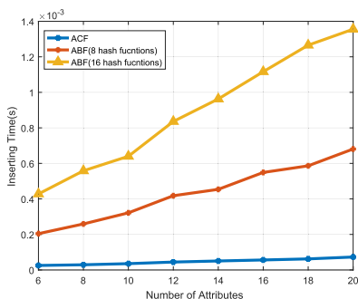
FIGURE 6. Attribute inserting time between ACF & ABF.
