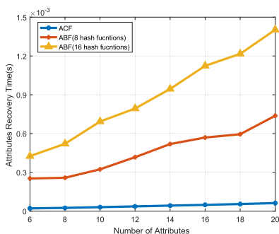
FIGURE 7. Attribute recovery time between ACF & ABF.
