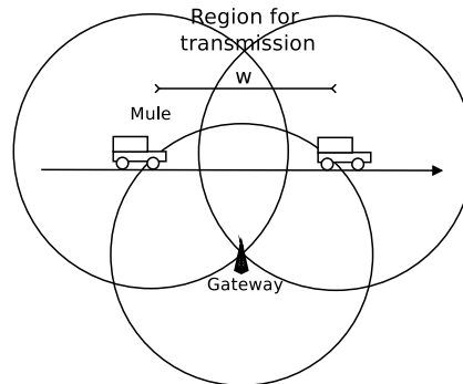
FIGURE 4. Gateway/Mule communication range.
