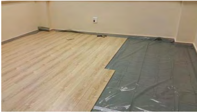
FIGURE 16. Installation of the sensor floor in the UJAmI smart lab.
