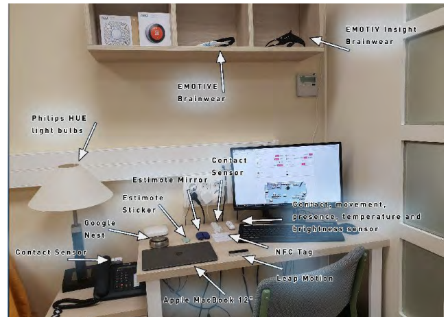
FIGURE 13. Workspace in the UJAmI smart lab.
