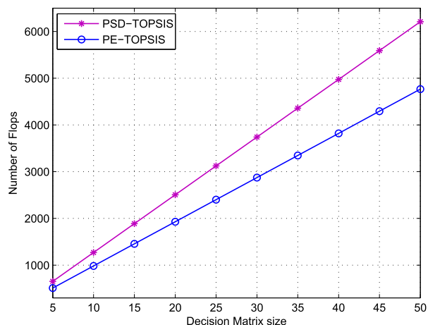
FIGURE 11. Complexity analysis.
