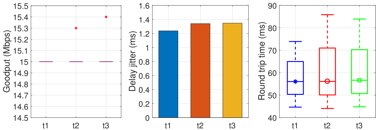
FIGURE 20. Flexible RAN deployment impacts on good-put, delay jitter and RTT.
