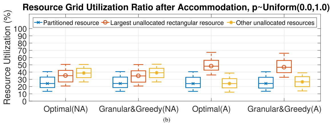
FIGURE 14. Performance of different slice prioritization policies and resource abstraction in resource accommodation. (a) Traffic arrival ratio p \sim \text{Uniform}(0.65, 1.0) . (b) Traffic arrival ratio p \sim \text{Uniform}(0.0, 1.0) .
