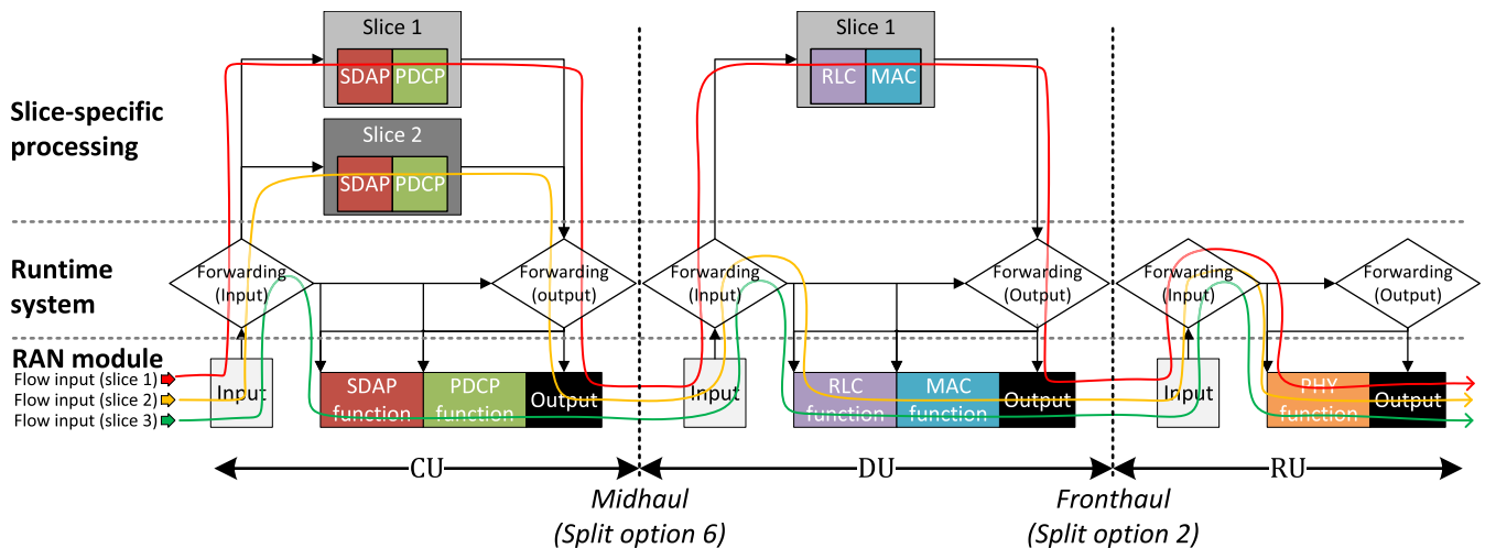
FIGURE 9. UP forwarding path in three-tier disaggregated RAN (CU, DU, RU).
