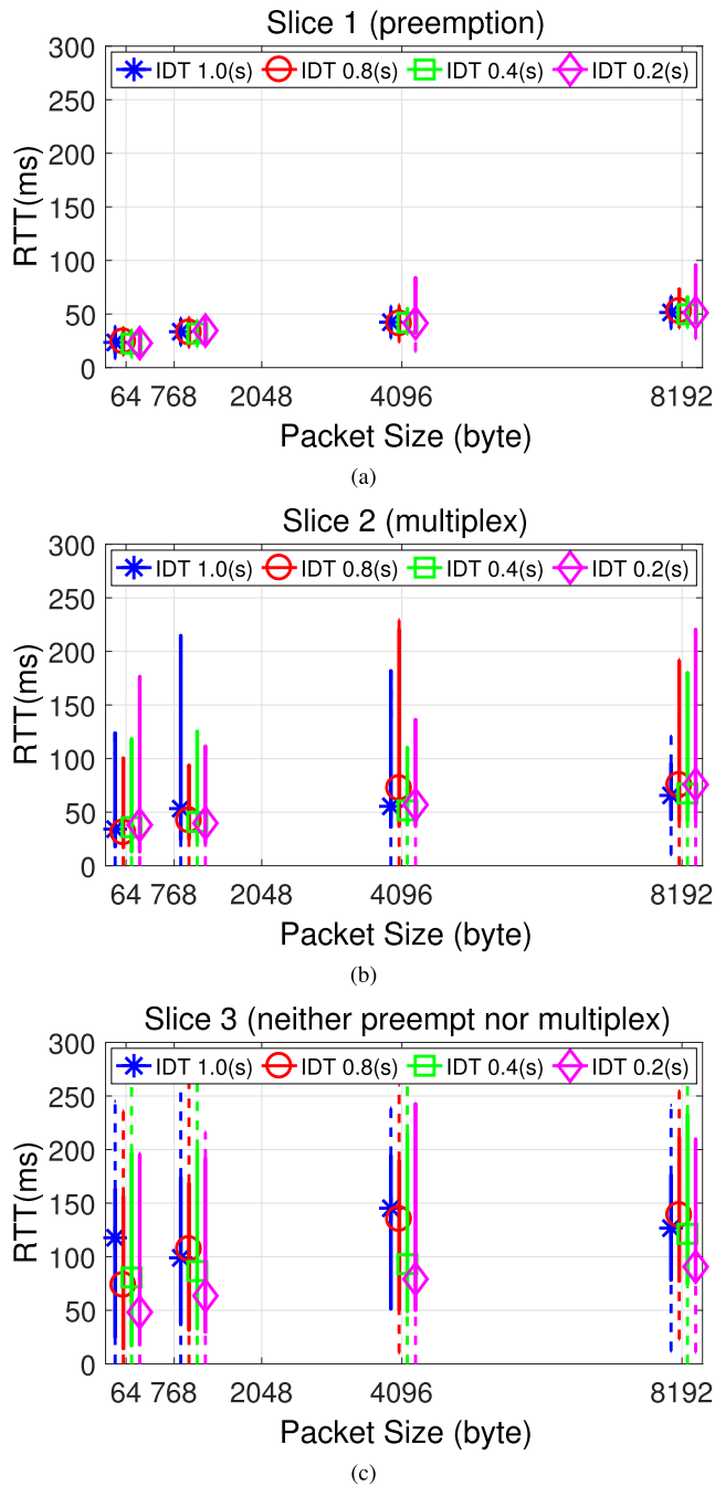
FIGURE 18. Impact of preemption and multiplexing on RTT. (a) Slice 1. (b) Slice 2. (c) Slice 3.
