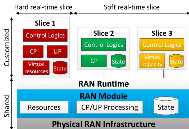
FIGURE 2. High-level architecture of RAN runtime slicing system.
