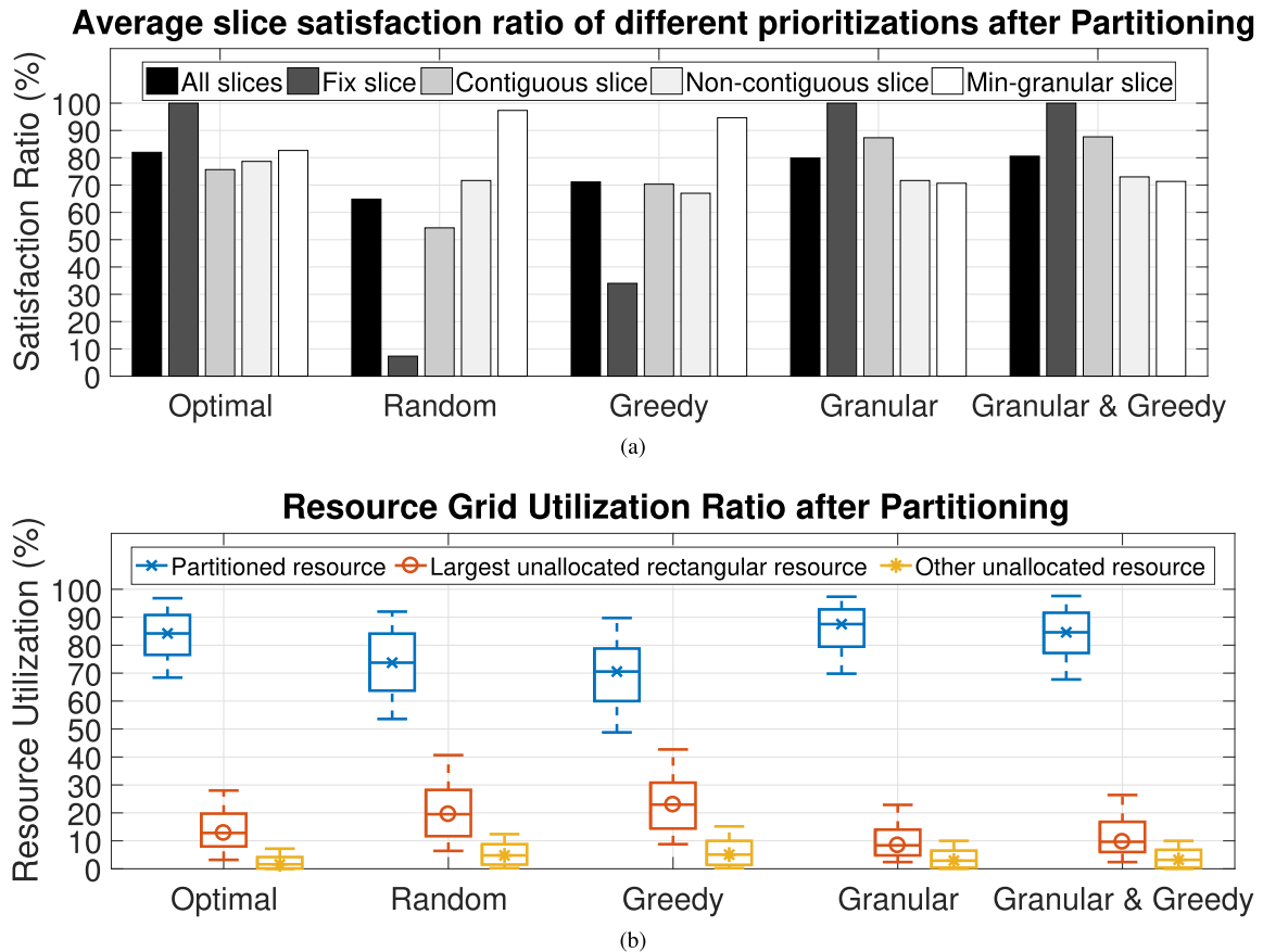
FIGURE 13. Performance of different slice prioritization policies in resource partitioning. (a) Average slice satisfaction ratio. (b) Resource grid occupation ratio.
