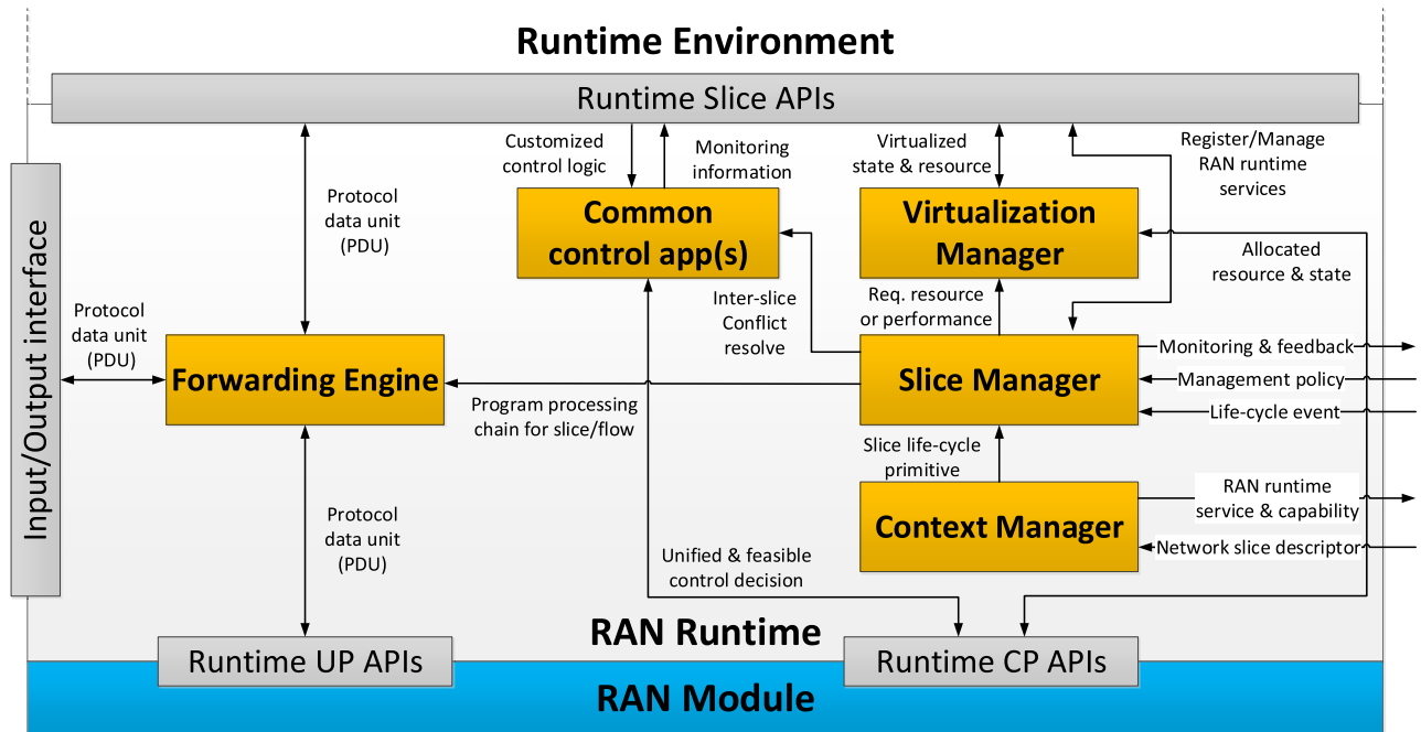
FIGURE 10. Message flows between RAN runtime services.
