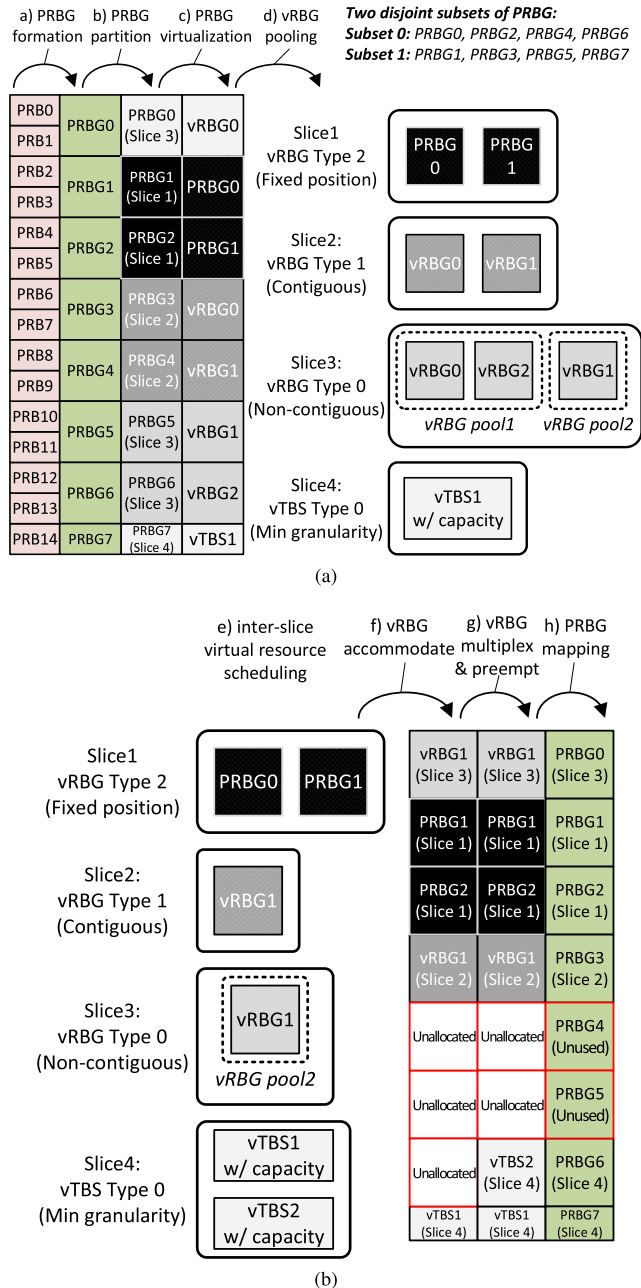
FIGURE 7. Different stages for virtualized resources slicing. (a) Stages partition PRB to vRBG pool. (b) Stages accommodate vRBG to PRBG.
