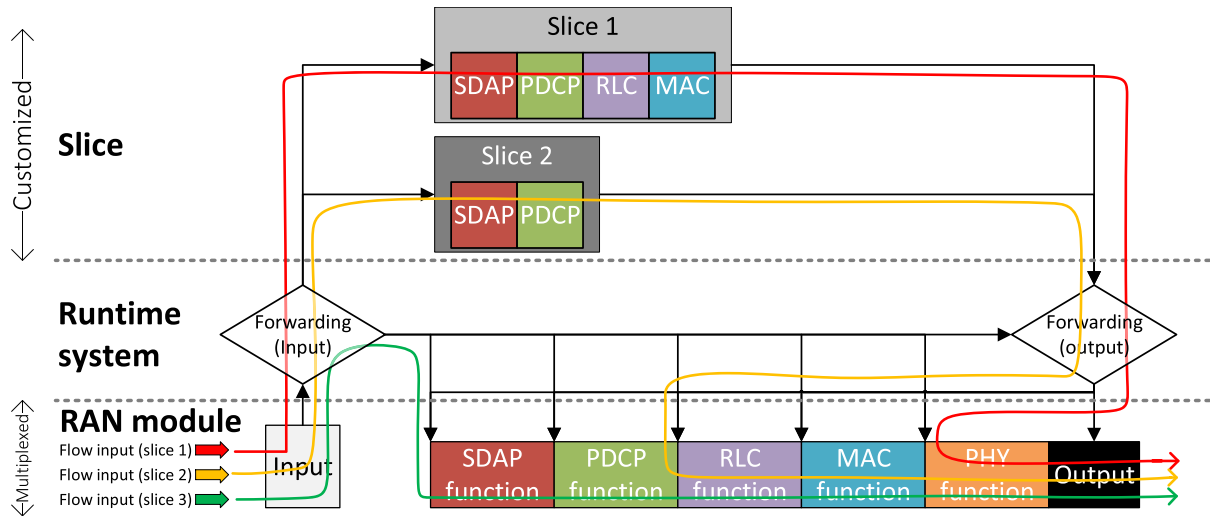
FIGURE 8. Forwarding engine and UP processing chain.
