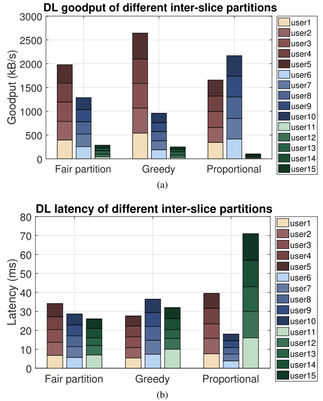
FIGURE 17. User performance of dynamic inter-slice partitioning. (a) Per-user average Good-put. (b) Per-user average latency.
