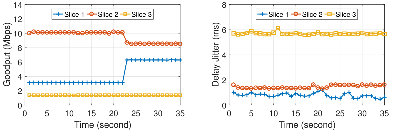
FIGURE 19. Impact of preemption and multiplexing on good-put and delay jitter.
