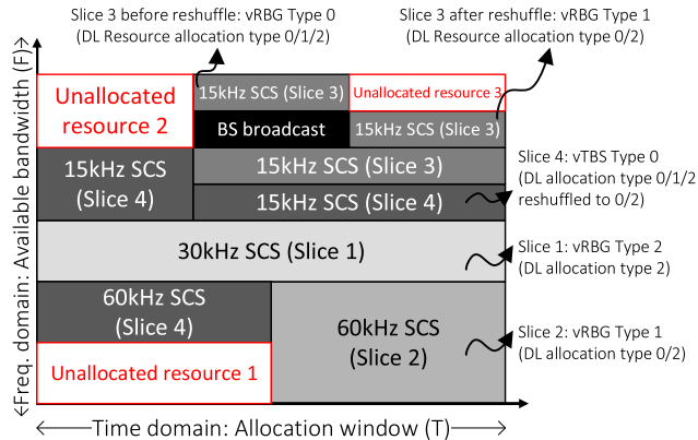
FIGURE 5. Resource partition with different abstraction types.
