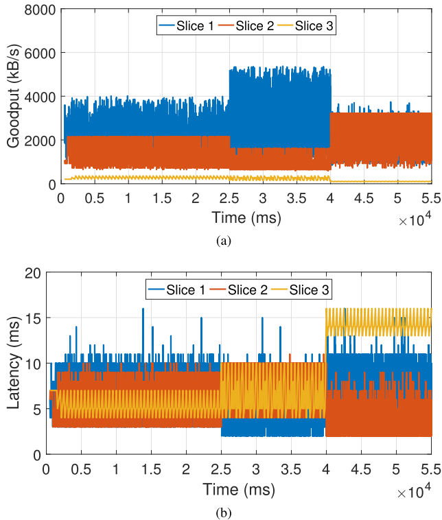
FIGURE 16. Slice performance of dynamic inter-slice partitioning. (a) Aggregated good-put. (b) Average latency.
