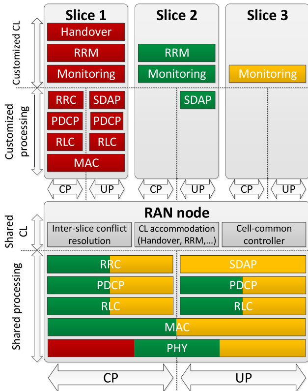
FIGURE 3. Examples for three instantiated slices.
