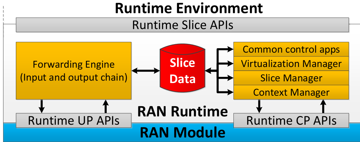
FIGURE 4. Architecture of the RAN runtime slicing system.
