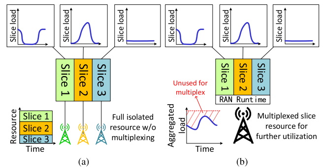
FIGURE 6. Multiplexing of slice resources. (a) Without resource multiplexing. (b) With resource multiplexing.
