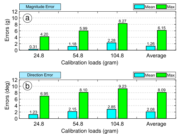
FIGURE 11. Mean and maximum errors in the magnitude (a) and direction (b) of the measured loads across three repetitive trials for the three known loads of 24.8, 54.8, and 104.8 grams as well as errors across all trials and loads during one turn rotation experiment.
