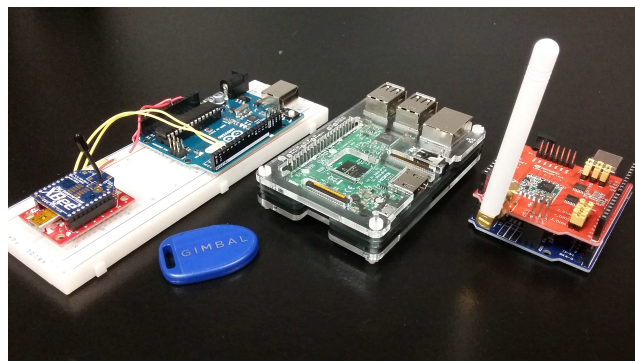
FIGURE 5. Equipment used in setting up the experiments. From left to right: Zigbee (Arduino Uno with Series 2 XBee), BLE (Gimbal Series 10 Beacon), WiFi (Raspberry Pi 3 Model B), LoRaWAN (Arduino Uno with Dragino LoRa Shield).
