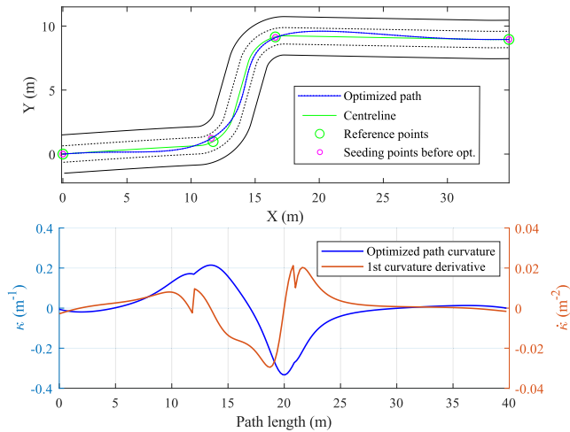
FIGURE 13. Results of test 1:D:5:LA-CE-J1:LOS-NM-J1:11:11. Scenario and final optimized path (top) and curvature of the final path and its first derivative (bottom).
