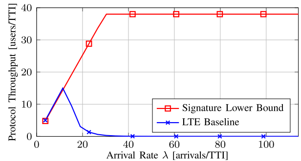
FIGURE 6. Protocol throughput for signature based access with 216 preambles.
