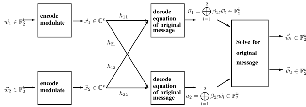
FIGURE 19. Toy example describing the main processing blocks for the 2 transmitters x 2 mini base stations case.
