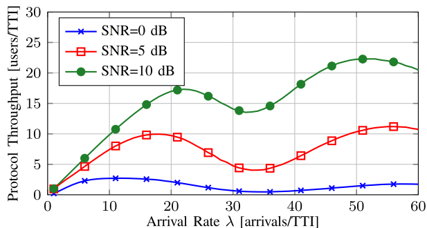
FIGURE 12. Protocol throughput for CSMUD.
