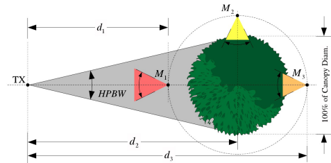
FIGURE 10. Measurement geometry for input parameter extraction.
