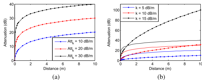
FIGURE 2. Attenuation given by the propagation model for various: a) Att_k and b) k values.
