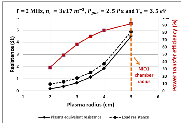
FIGURE 16. Plasma equivalent resistance, load resistance and power transfer efficiency variation with plasma radius using multi-filament model.
