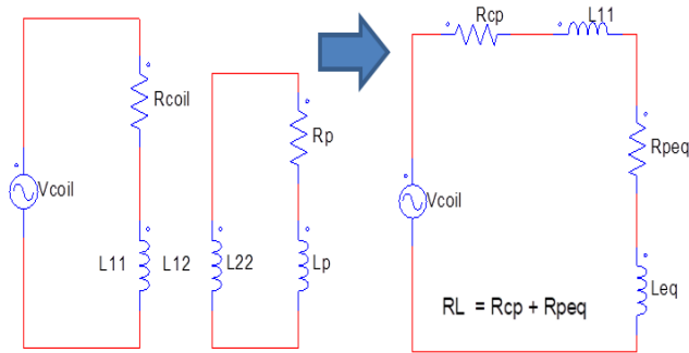
FIGURE 3. Transformer model (left hand side) - Equivalent electrical scheme of the driver (right hand side) including the plasma.
