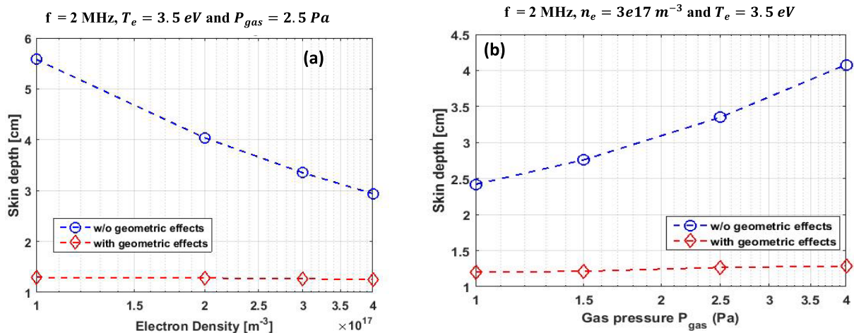
FIGURE 9. Skin depth variation with (a) electron density and (b) gas pressure.
