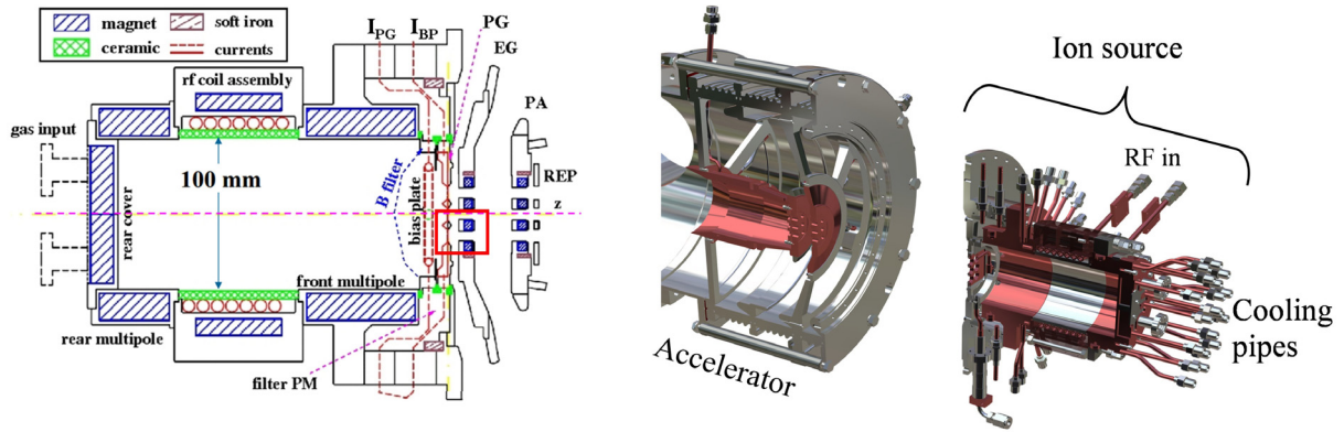
FIGURE 6. NIO1 ion source: schematic (left) and 3D drawing cut-view (right) of the driver and the accelerator region.
