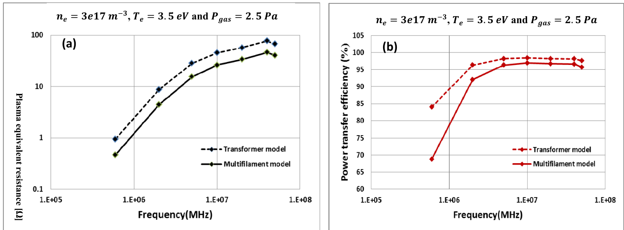
FIGURE 13. (a) Plasma equivalent resistance variation with frequency and (b) Power transfer efficiency variation with frequency.
