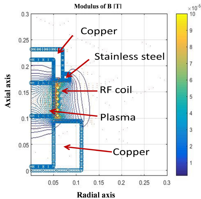
FIGURE 10. Schematic of the 2D axis-symmetry model of the driver of the NIO1 ion source.
