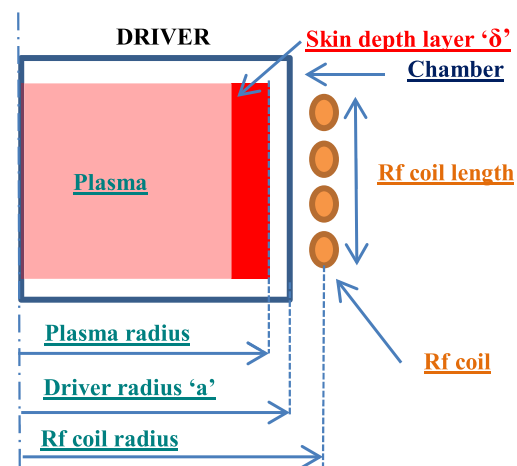
FIGURE 2. Schematic of the plasma within the driver.
