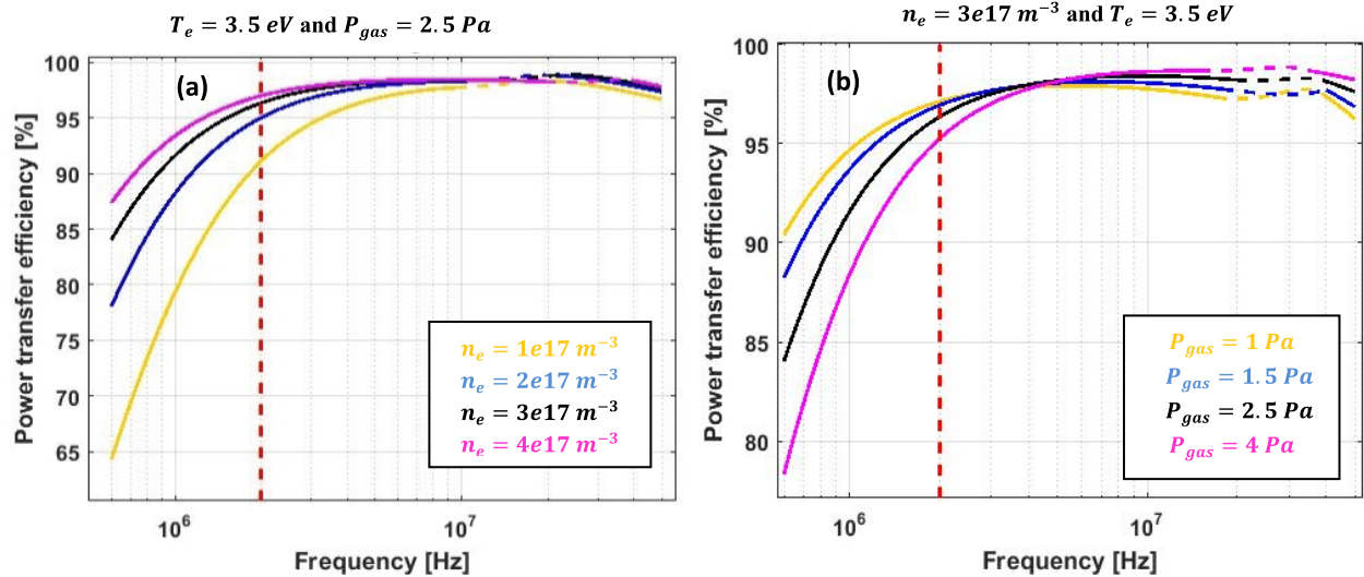
FIGURE 12. Variation of power transfer efficiency with frequency for different (a) electron densities and (b) gas pressure.
