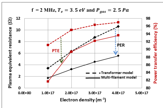
FIGURE 14. Plasma equivalent resistance and power transfer efficiency variation with electron density.
