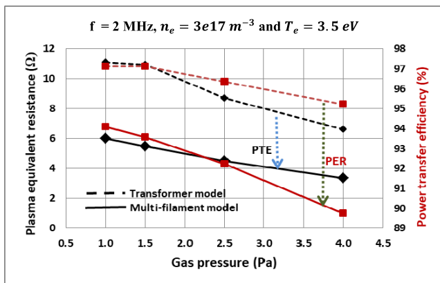
FIGURE 15. Plasma equivalent resistance and power transfer efficiency variation with gas pressure.
