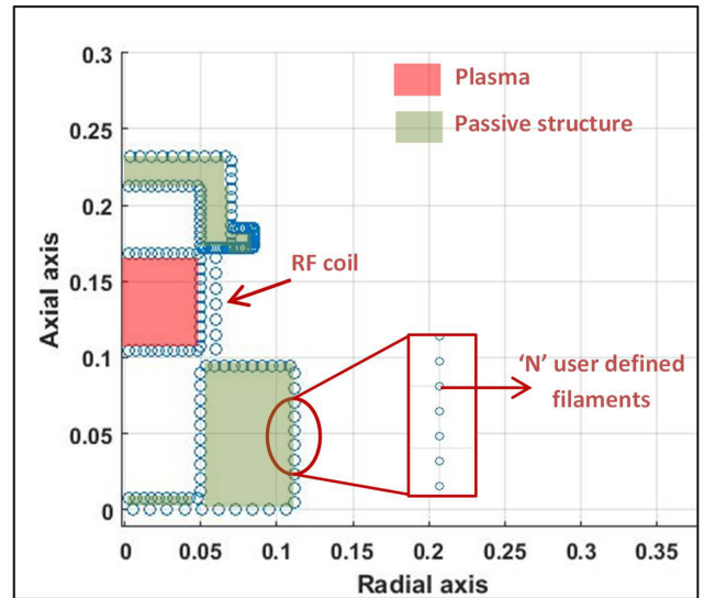
FIGURE 4. Representation of the 2D multi-filament model with 'N' user defined current filaments for the driver of NIO1 ion source.
