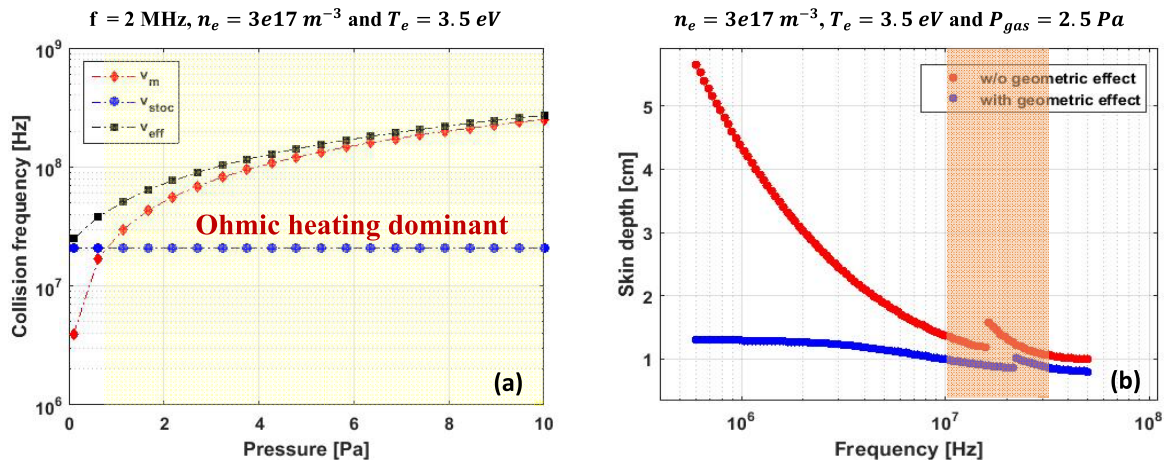
FIGURE 8. Variation of (a) effective, ohmic and stochastic collision frequency with gas pressure and (b) skin depth with applied frequency.
