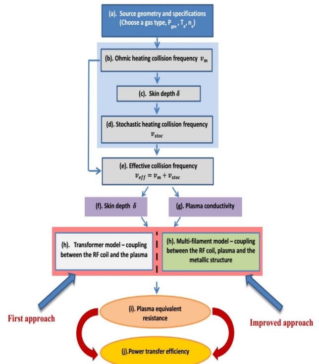
FIGURE 1. Methodology to calculate the power transfer efficiency in an IC RF ion source.
