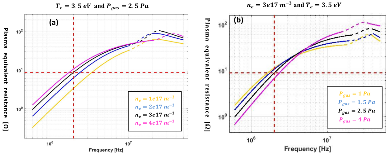
FIGURE 11. Variation of plasma resistance with frequency for different (a) electron density and (b) gas pressure.
