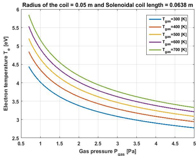
FIGURE 7. Estimation of electron temperature with gas pressure.
