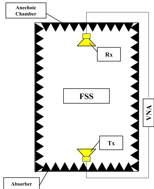
FIGURE 10. Measurement setup for FSS measurement.
