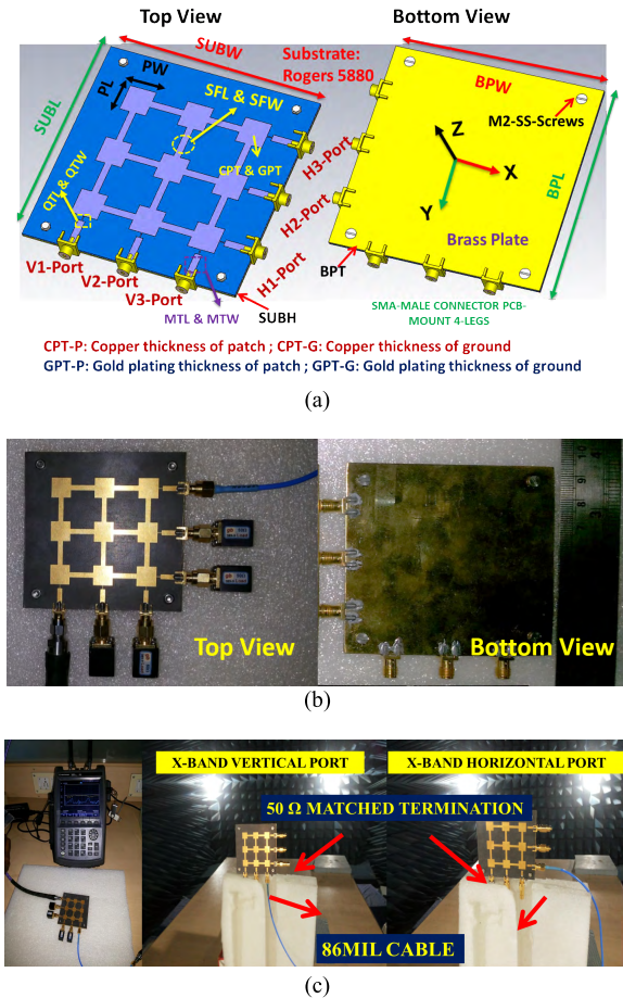
FIGURE 1. The geometry of the proposed 6-port 3 × 3 planar array (a) CST model (b) Fabricated prototype (c) S-parameters and radiation pattern measurement setup in anechoic chamber.
