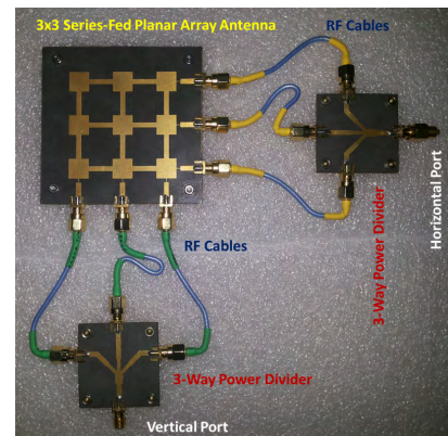
FIGURE 7. Combined V-ports and H-ports with 3-way power divider for maximum gain.
