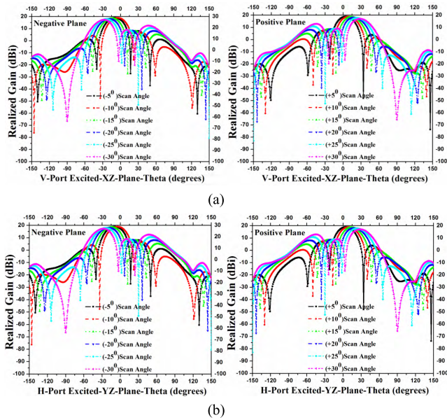
FIGURE 8. Scan angle patterns of xz-plane for different progressive phase shift (a) V-Polarization, (b) H-Polarization.
