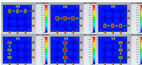
FIGURE 2. The surface current distribution at 9.65 GHz for all ports.
