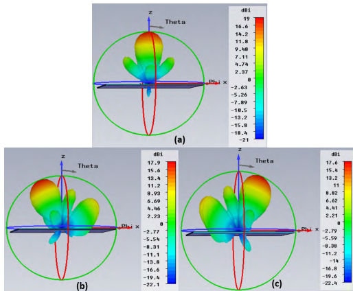
FIGURE 9. 3D far-field gain (a) Broadside direction ( \phi = 0^\circ & \theta = 0^\circ ), (b) Elevation tilt angle ( \phi = 0^\circ & \theta = -25^\circ ), (c) Elevation tilt angle ( \phi = 0^\circ & \theta = +25^\circ ).
