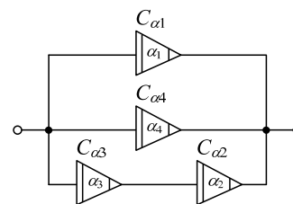
FIGURE 8. Second series-parallel interconnection of arbitrary-order FoCs (#10).
