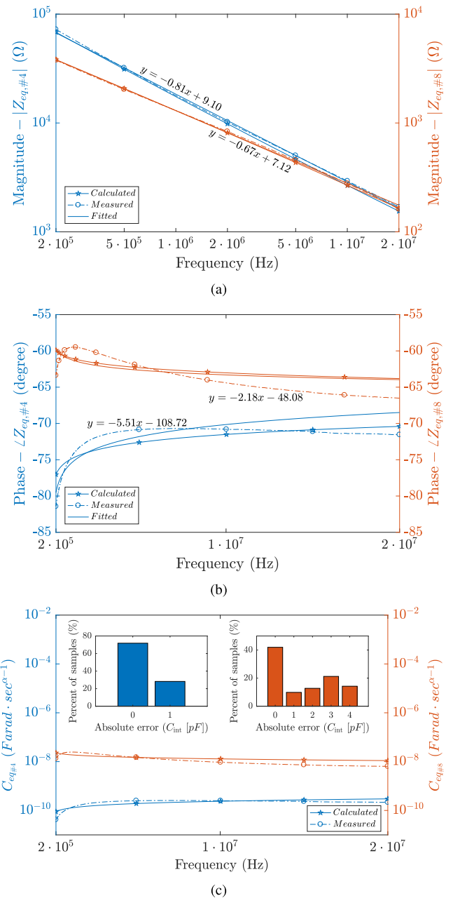
FIGURE 10. Comparison of (a) magnitude, (b) phase, and (c) pseudo-capacitance versus frequency of three arbitrary-order FoCs connected in series (#4 - blue color) and parallel (#8 - orange color).
