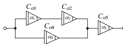
FIGURE 7. First series-parallel interconnection of arbitrary-order FoCs (#9).
