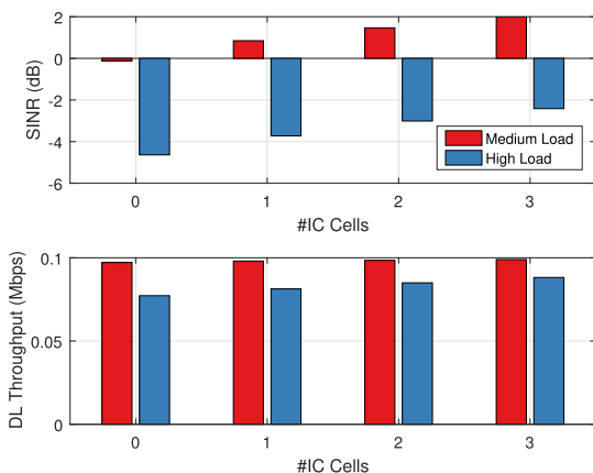
FIGURE 14. Average UAV DL SINR and throughput vs. number of interfering cells whose signal was canceled. UAVs account for 1% users in the network and fly at constant height of 120 m.
