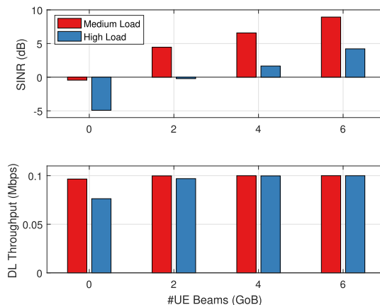
FIGURE 9. Average UAV DL SINR and throughput vs. number of antenna beams. UAVs account for 1% users in the network and fly at constant height of 120 m.
