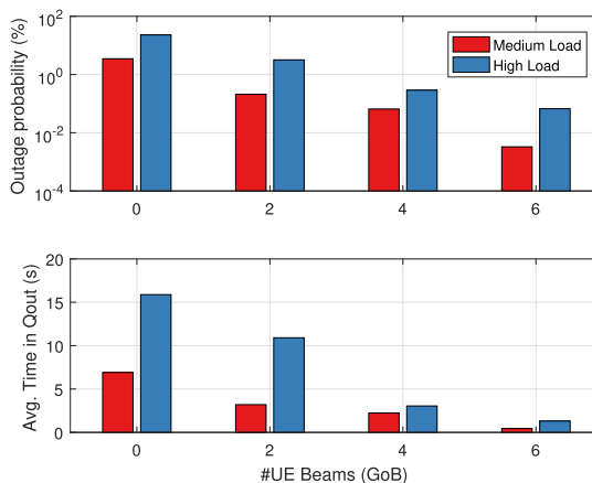
FIGURE 10. UAV outage probability and average time in Q_{out} vs. number of antenna beams. UAVs account for 1% users in the network and fly at constant height of 120 m.
