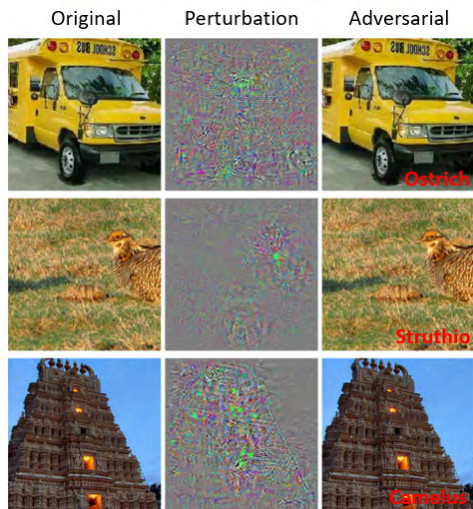
FIGURE 2. Illustration of adversarial examples generated using [22] for AlexNet [9]. The perturbations are magnified 10x for better visualization (values shifted by 128 and clamped). The predicted labels of adversarial examples are also shown.
