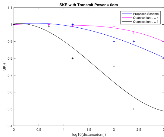
FIGURE 3. Successful Key Reconciliation Rate versus Node Distance at 0dm for proposed scheme and for the scheme proposed by Wilhelm et. al [4] at different quantisation levels.
