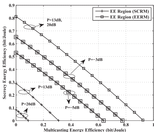
FIGURE 7. EE regions in PHY-SI [52].
