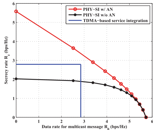
FIGURE 4. Secrecy rate regions with and without AN [34].
