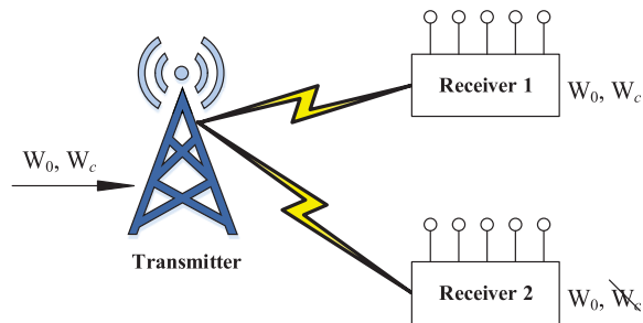
FIGURE 1. PHY-SI of multicast and confidential unicasting.
