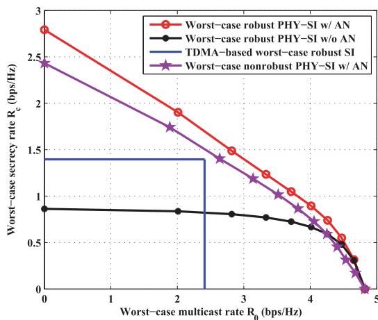
FIGURE 6. Worst-case secrecy rate regions with and without AN [34].
