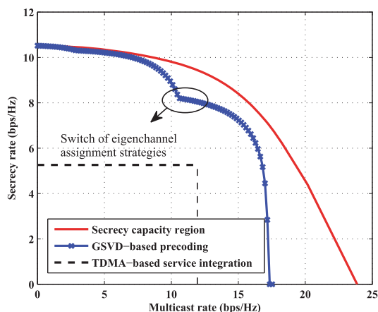
FIGURE 5. Secrecy rate regions by message decoupling [41].
