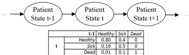
FIGURE 4. Dynamic Bayesian network.
