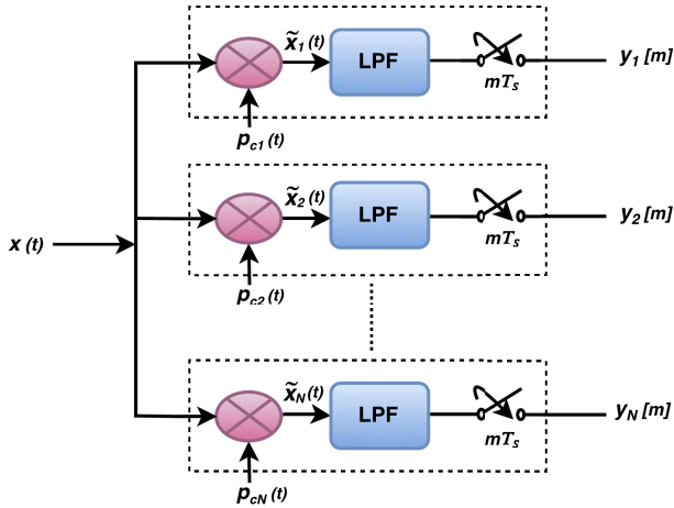
FIGURE 5. CS acquisition using MWC technique.
