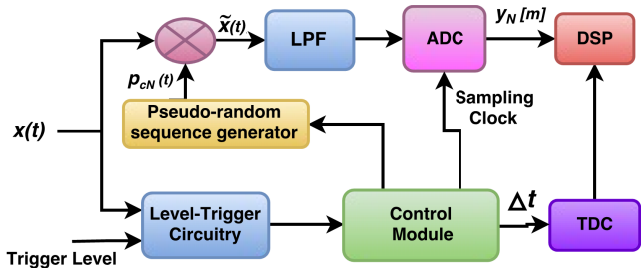
FIGURE 10. CS acquisition using RT-MWCS technique.
