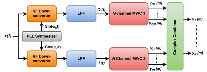
FIGURE 11. CS acquisition using QAIC technique.
