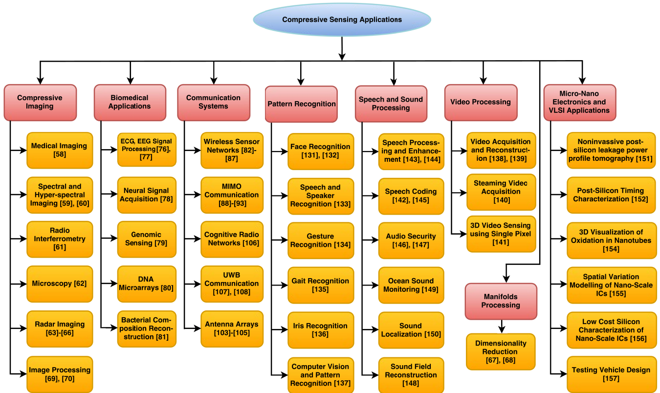
FIGURE 19. Major applications of CS.
