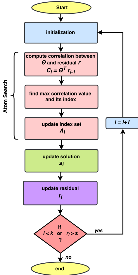
FIGURE 15. Algorithmic steps of serial greedy algorithms.
