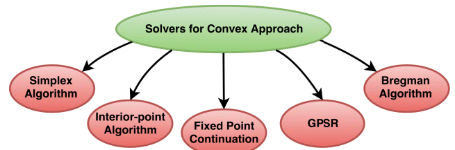
FIGURE 13. Solvers used for solving convex optimization problem of CS reconstruction.
