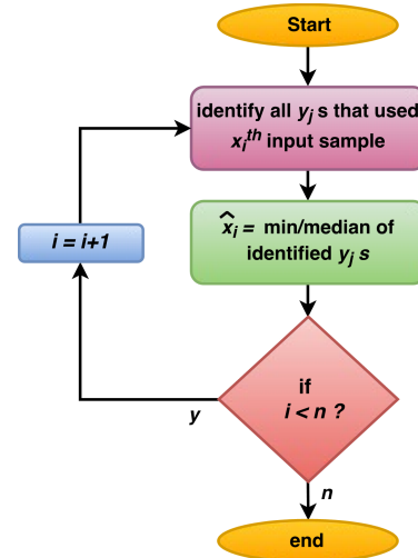
FIGURE 17. Algorithmic steps of count-min/median strategies used by algorithms under combinatorial approach.
