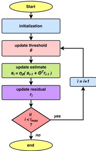
FIGURE 16. Algorithmic steps of AMP algorithm.
