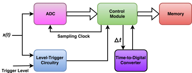
FIGURE 9. CS acquisition using RES technique.
