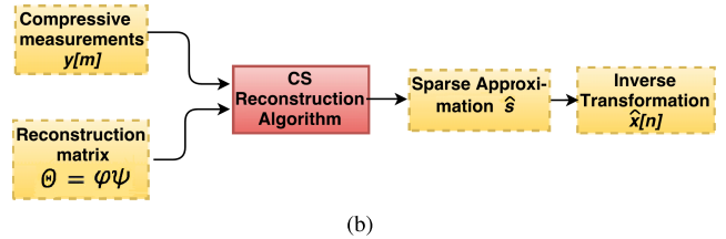
FIGURE 3. CS Model: (a) acquisition model, (b) reconstruction model.
