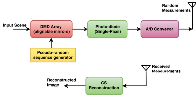
FIGURE 20. Block diagram of single-pixel camera.
