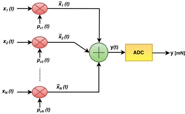
FIGURE 8. CS acquisition using CMUX technique.
