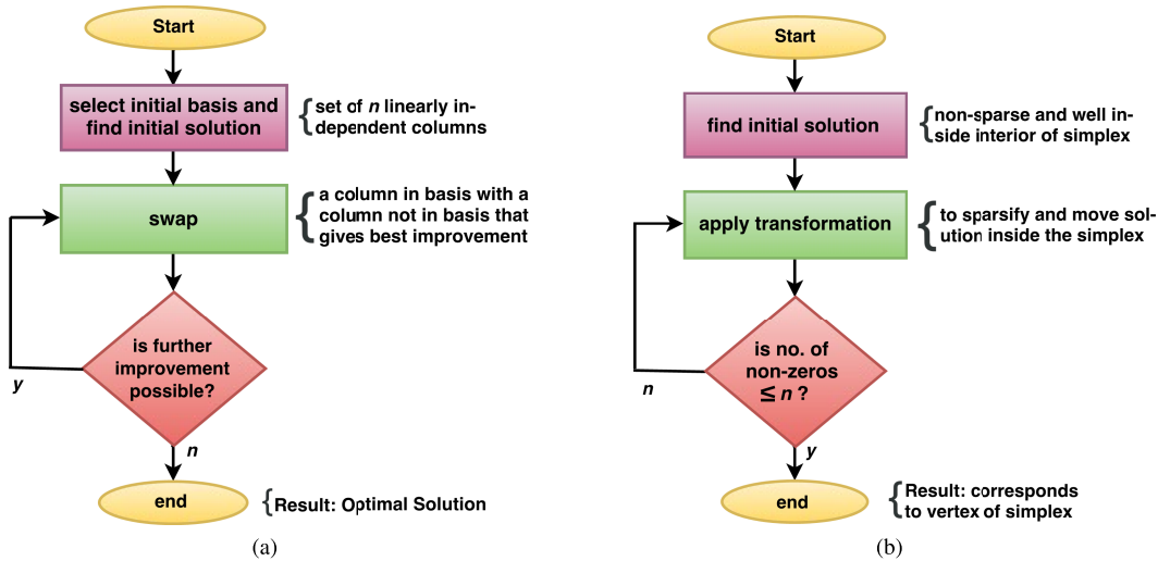
FIGURE 14. Algorithmic steps of solvers for basis pursuit namely: (a) simplex method and (b) interior-point method.
