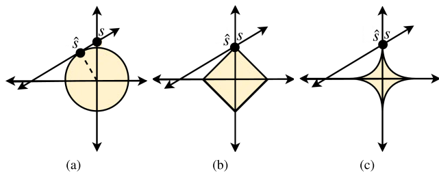
FIGURE 18. Example to illustrate sparse solution approximation using unit normed-balls in 2-D space: (a) \ell_2 -ball, (b) \ell_1 -ball, (c) \ell_{1/2} -ball.
