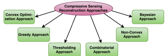
FIGURE 12. CS reconstruction approaches.
