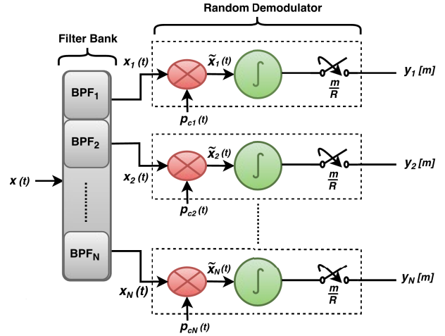
FIGURE 6. CS acquisition using RMPI technique.
