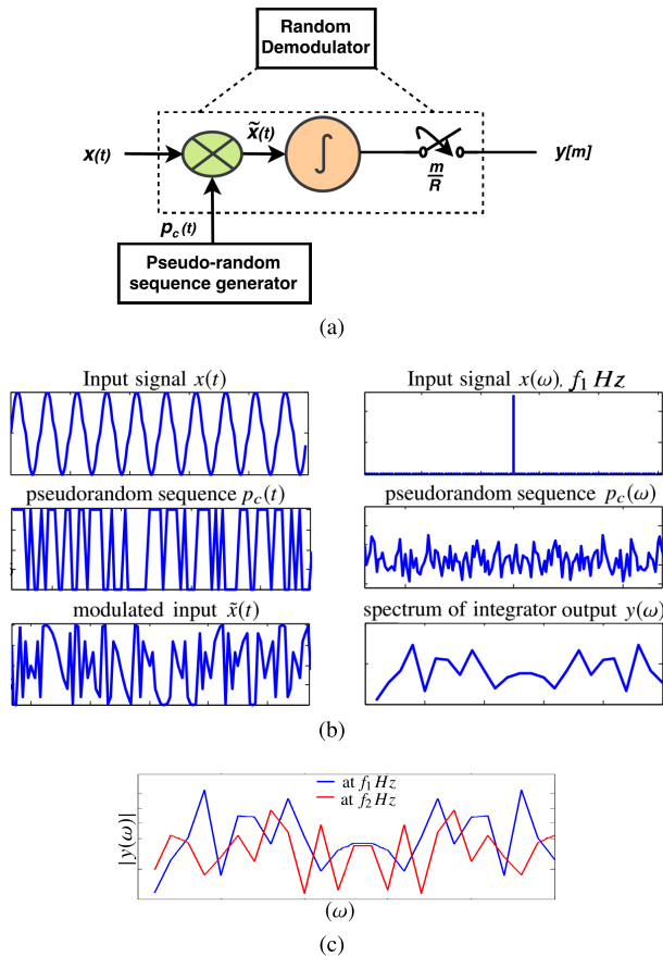
FIGURE 4. CS acquisition using RD technique. (a) Block diagram of RD. (b) Input-output waveforms generated at each stage. (c) Unique frequency signatures obtained after integrator stage for two different frequencies f_1 Hz and f_2 Hz.
