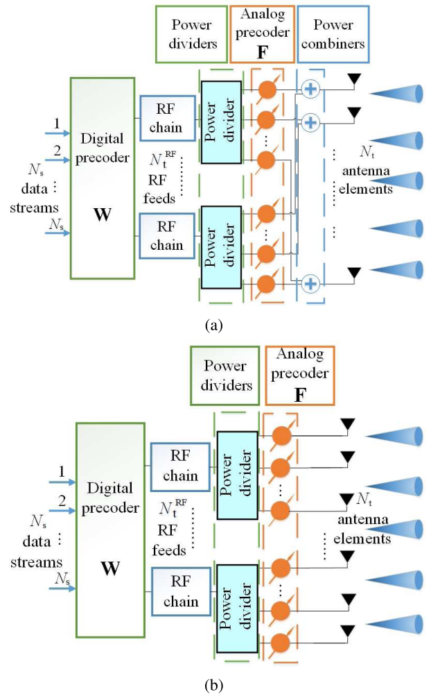
FIGURE 1. Conventional hybrid precoding architectures with phased array antennas: (a) full-connected model, and (b) sub-connected model, where the transmitter employs N_t antennas with N_t^{RF} (\leq N_t) RF chains to support N_s (\leq N_t^{RF}) independent data streams, and typically N_t^{RF} \ll N_t .
