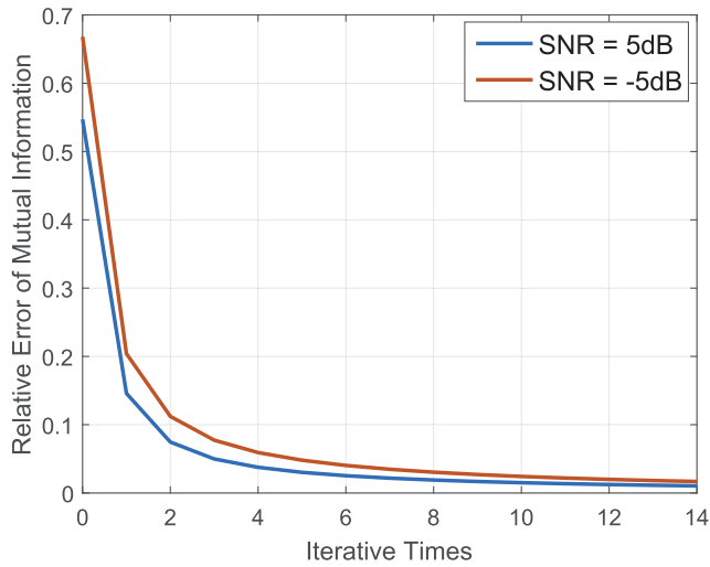
FIGURE 3. Convergence performance of Algorithm 1 given two different values of SNR, where N_t = 8 \times 8 , N_r = 4 \times 4 , N_t^{RF} = 8 , and N_s = 4 .
