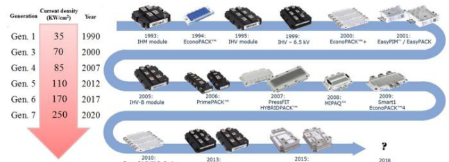
FIGURE 3. Development power density in generation of IGBTs.
