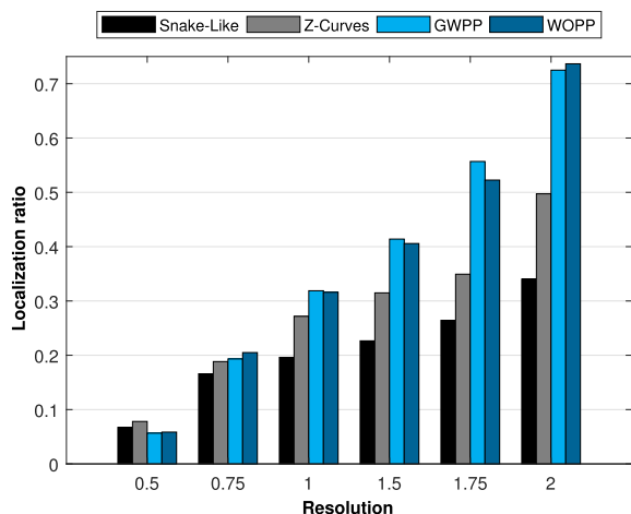
FIGURE 13. Localization ratio versus the resolution of all mobility models in both WCL and WCWL.
