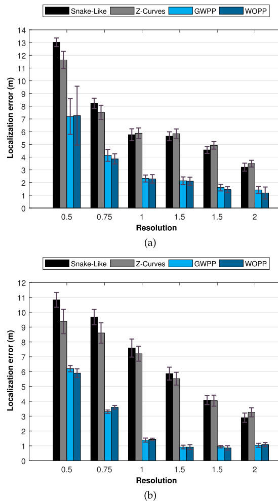
FIGURE 10. Average localization errors and resolution in (a) WCL, and (b) WCWCL.
