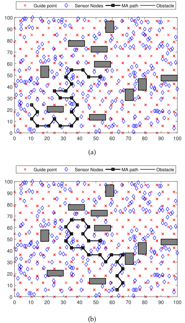
FIGURE 6. The obstacle-avoidance path planning of the two models in (a) GWPP, and (b) WOPP.
