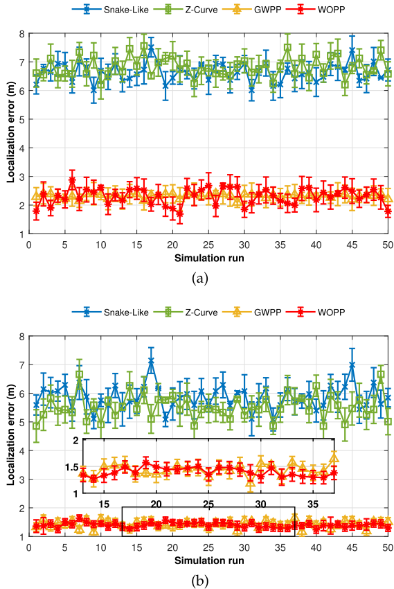
FIGURE 8. Localization errors of all mobility models in (a) WCL, and (b) WCWCL, ( d_{max} = 140 , R = 1 ).
