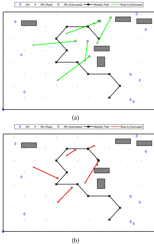
FIGURE 7. Example of the localization estimation when the same nodes deployment and the same MA movement are used in (a) WCL, and (b) WCWCL.
