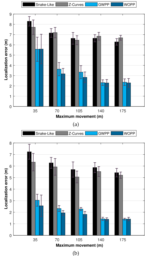
FIGURE 9. Average localization errors versus maximum movement in (a) WCL, and (b) WCWCL.
