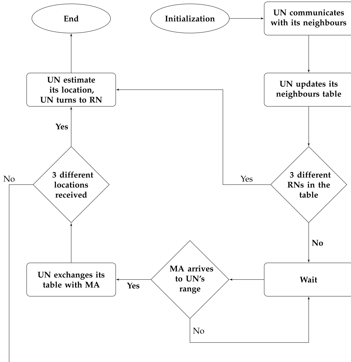
FIGURE 4. The node localization process in the UN.
