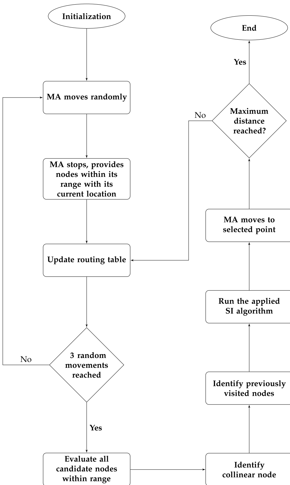
FIGURE 5. The movement and node localization process in the MA.
