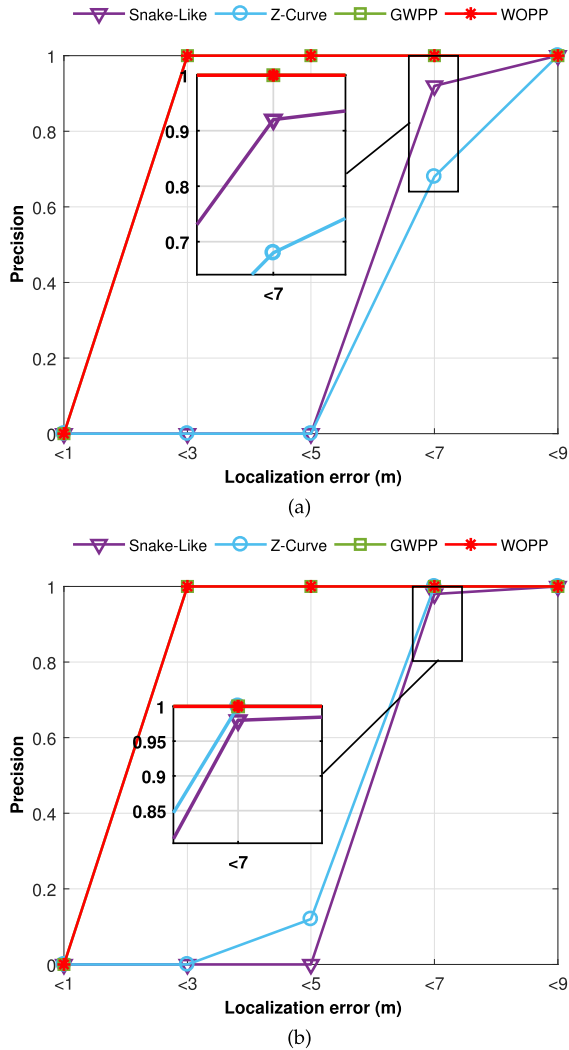
FIGURE 11. Precision of all mobility models versus the localization error in (a) WCL, and (b) WCWCL, ( d_{max} = 140 , R = 1 ).
