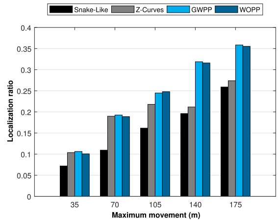
FIGURE 12. Localization ratio versus the maximum movement distance of all mobility models in both WCL and WCWCL.
