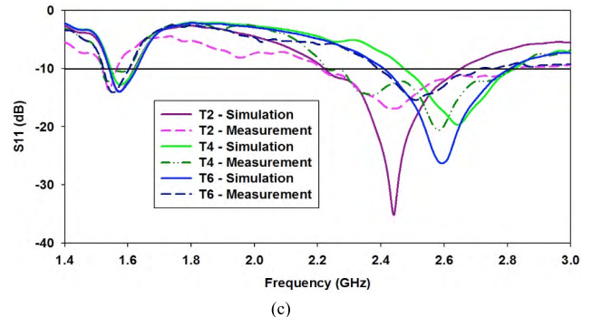
FIGURE 10. Simulated and measured reflection coefficients for different configurations: (a) T1 and T3, (b) T5 and T7 and (c) T2, T4 and T6.
