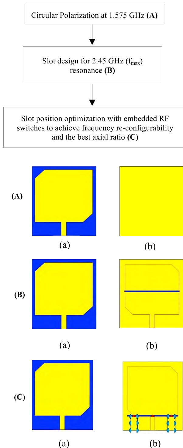
FIGURE 1. The design methodology to achieve CP and frequency specified reconfigurable antenna. a) Front view and b) Back view.
