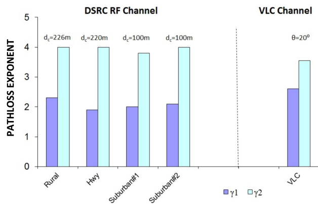
FIGURE 1. Example path loss model from empirical measurements.
