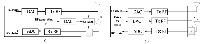
FIGURE 5. The non-adaptive extra RF chain circuitry for SIC [37].
