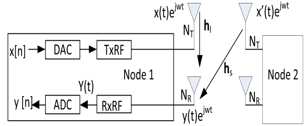
FIGURE 9. Full duplex system model.
