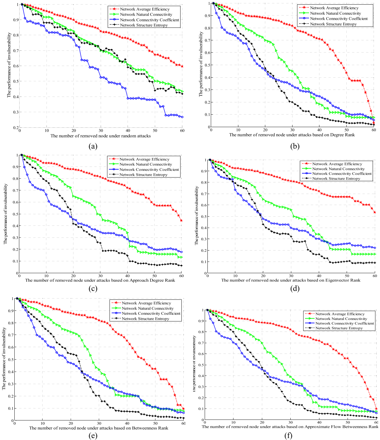
FIGURE 4. Effect of network invulnerability by different attacks.
