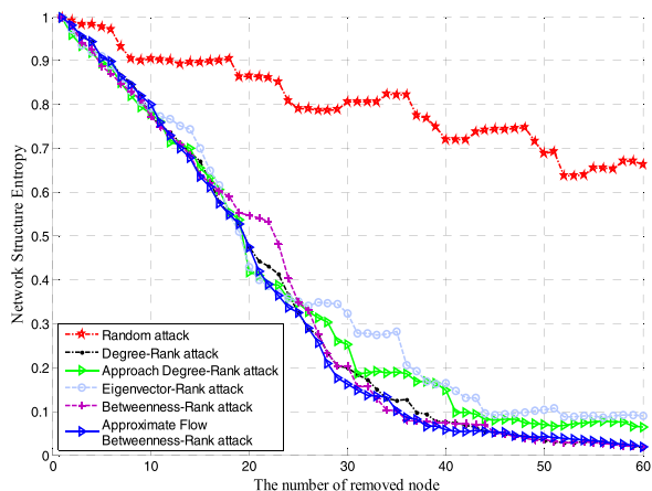
FIGURE 3. The effect of network structure entropy by different attacks.
