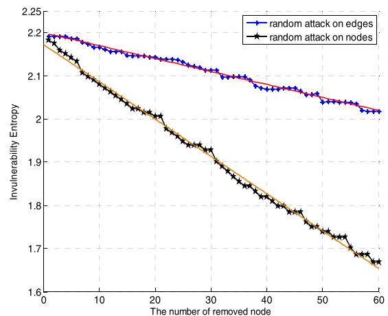
FIGURE 2. The changes of the node and edge structure entropy under random attack.
