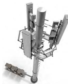
FIGURE 1. Configuration of a typical base station array for cellular coverage.
