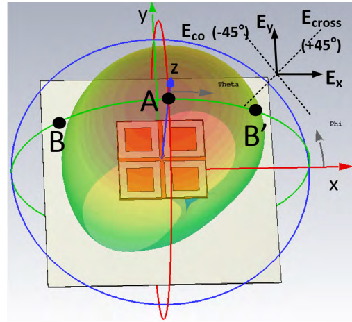
FIGURE 7. Schematic 3D radiation pattern of the proposed tightly-coupled cross-dipole.
