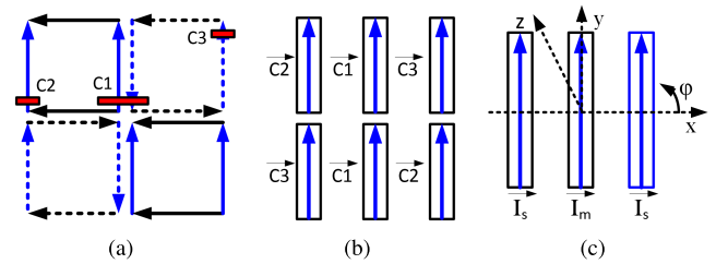
FIGURE 9. Representation of the current distributions. (a) Schematic for the tightly-coupled cross-dipole antenna. (b) Equivalent six-element dipole array for model-A. (c) Reduced, equivalent three-element dipole array model.
