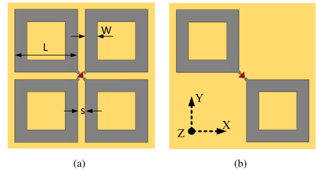
FIGURE 3. Cross-dipole geometry. (a) Model-A: tightly-coupled cross dipoles consisting of a driven dipole and a parasitic dipole. (b) Model-B: driven dipole only.
