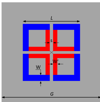
FIGURE 11. Revised and simplified cross-dipole configuration.
