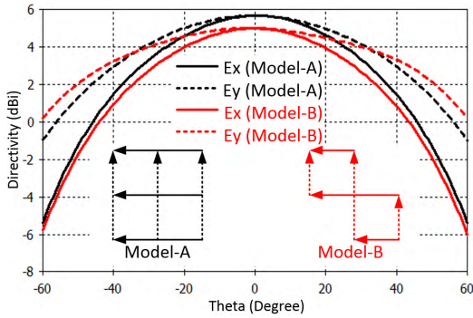
FIGURE 8. Comparison of x- and y-aligned radiation patterns of Models-A and -B.
