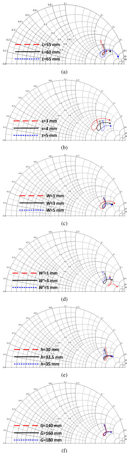
FIGURE 13. Input impedance plotted on the Z-Smith diagram for the parameters: (a) L , (b) s , (c) W , (d) W' , (e) h , and (f) G .
