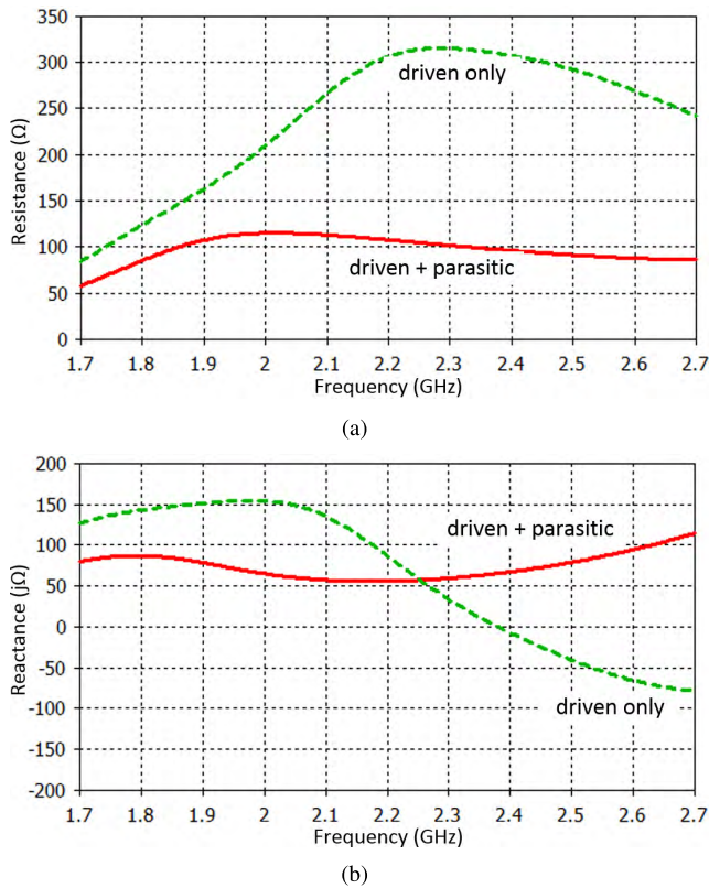
FIGURE 4. Variations of the impedance of Model-A and Model-B in the target band. (a) Resistance. (b) Reactance.
