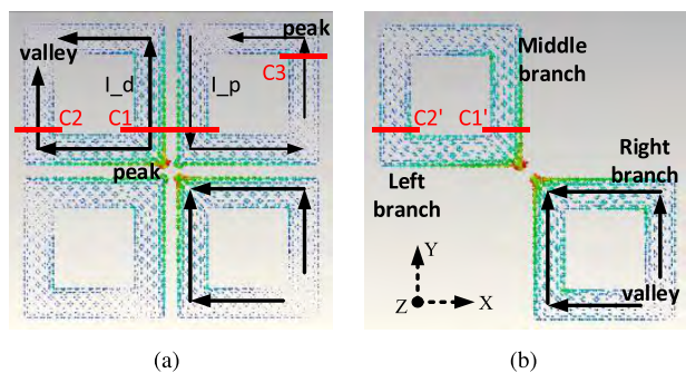
FIGURE 5. Current distributions on the traces of the models. (a) Model-A. (b) Model-B.
