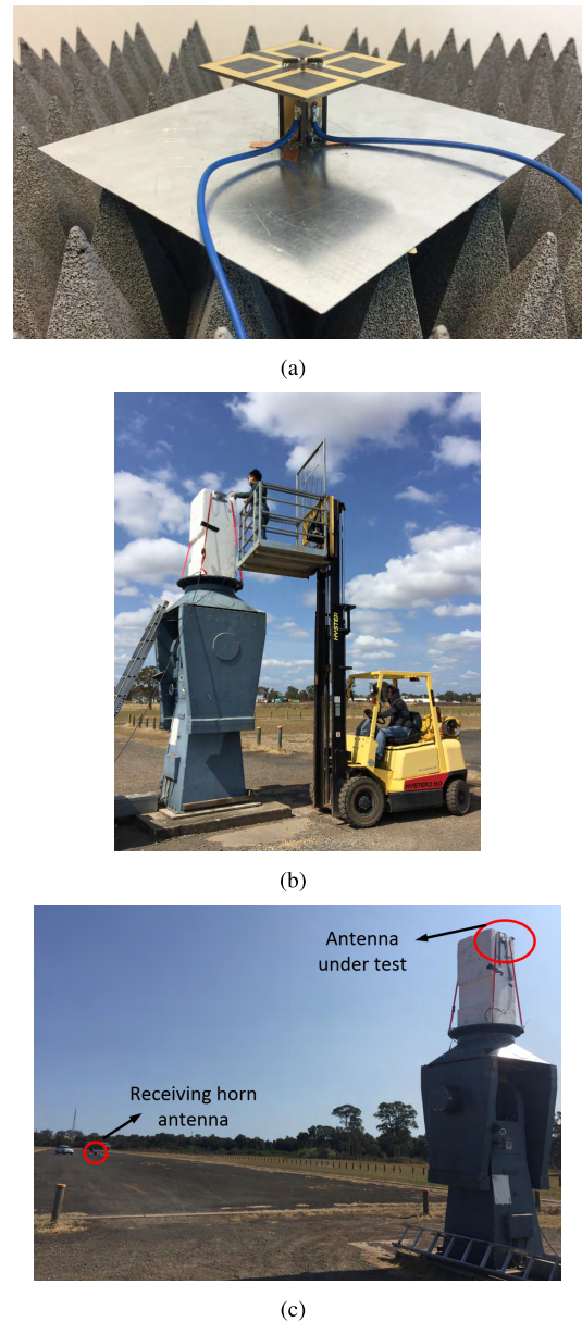
FIGURE 15. Photos of the antenna and measurement system. (a) Fabricated and assembled antenna prototype. (b) Mounting the antenna. (c) Antenna under test (AUT).
