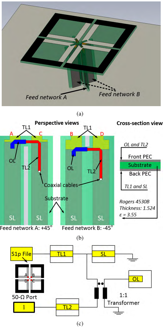
FIGURE 14. Optimized simplified cross-dipole antenna. (a) Perspective view. (b) Details of the two feed networks implemented using PCBs. (c) Circuit theory model of the matching circuit.
