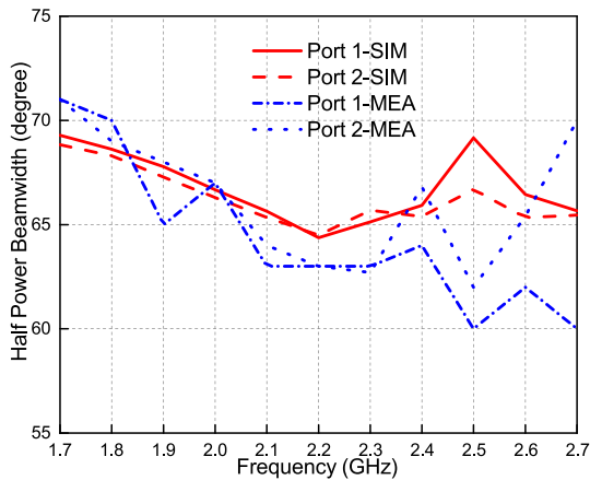
FIGURE 18. Simulated and measured HPBW for the two polarizations across the target band.
