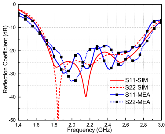
FIGURE 16. Simulated and measured reflection coefficients of the two ports.
