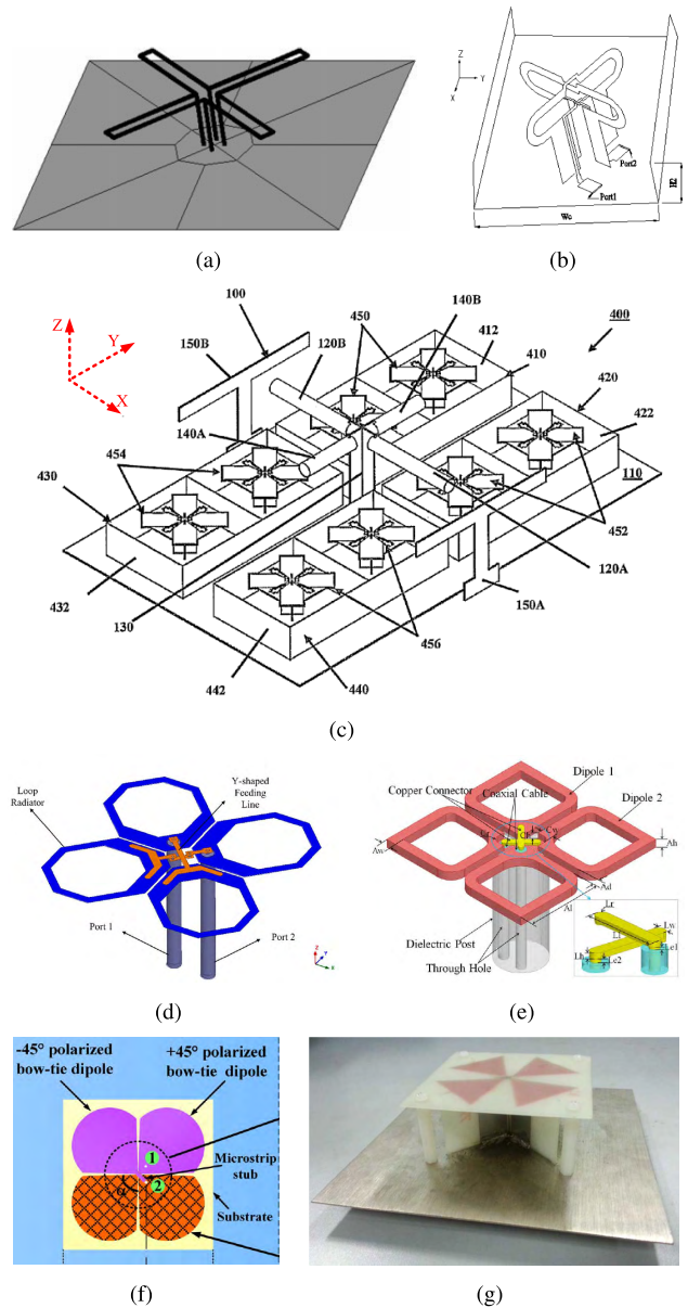
FIGURE 2. Configurations of dual-polarized cross-dipoles developed for base station applications reported in the literature. (a) Ref [7]. (b) Ref [8]. (c) Ref [9]. (d) Ref [10]. (e) Ref [11]. (f) Ref [12]. (g) Ref [13].
