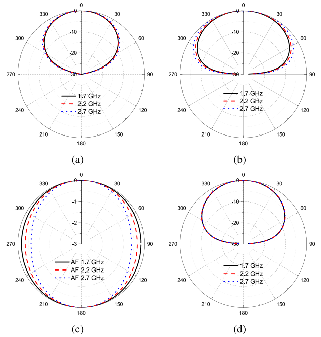
FIGURE 10. Simulated radiation patterns. (a) E-plane pattern and (b) H-plane pattern of a single half-wavelength dipole placed a quarter-wavelength above an infinite ground plane and oriented parallel to it. (c) Three-element array factor pattern alone. (d) Model-A-based cross-dipole radiation pattern.
