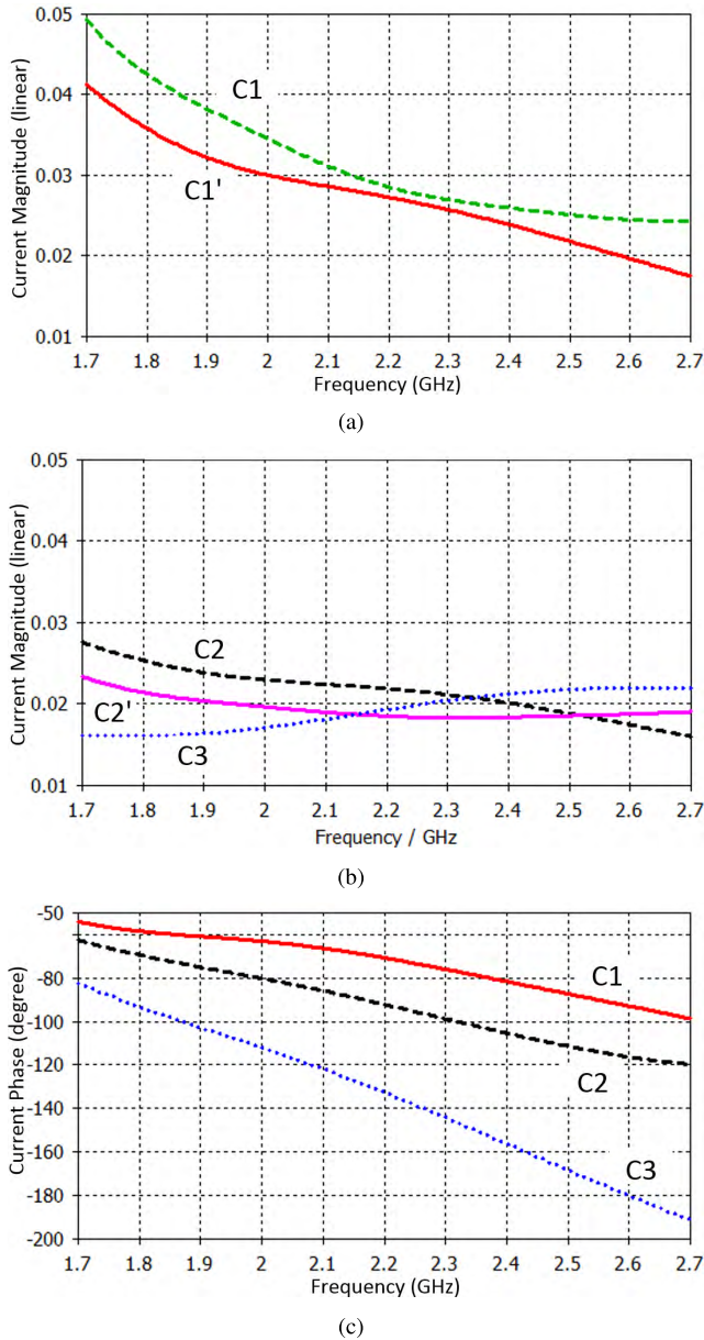
FIGURE 6. Simulated currents. (a) Current magnitude on the middle branches of Model-A and Model-B. (b) Current magnitudes on the side branches of Model-A and Model-B. (c) Current phases on three different branches of Model-A.
