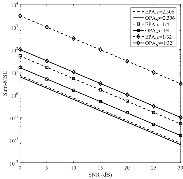
FIGURE 3. Sum-MSE versus receive SNR for three different values of \rho ( \leq \rho^o ) ( \alpha_{t,S} = 5dB , \alpha_{t,R} = \alpha_{r,R} = 1dB ).
