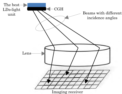
FIGURE 11. Imaging optical receiver with angular spatial mapping.
