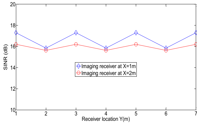
FIGURE 18. SINR of one beam of the adaptive CGH-VLC system at different locations of the imaging receiver along the y-axis and at x = 1 m and x = 2 m in room A when each beam operates at a data rate of 5 Gb/s.
