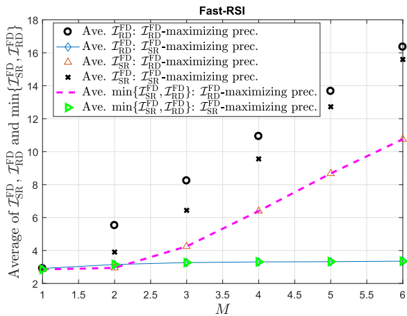
FIGURE 8. Average achievable rate of the source-relay link for the fast-RSI case under \mathcal{I}_{RD}^{FD} -maximizing and \mathcal{I}_{SR}^{FD} -maximizing precoders. The average of the minimum between the achievable rate of the source-relay and relay-destination links is plotted for both cases of \mathcal{I}_{RD}^{FD} -maximizing and \mathcal{I}_{SR}^{FD} -maximizing precoders.
