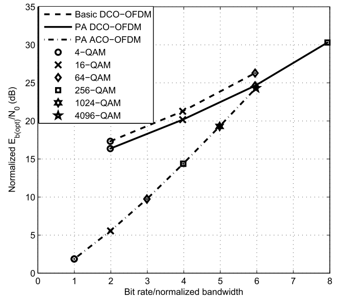
FIGURE 7. E_{b(\text{opt})}/N_0 against bit rate/normalized bandwidth for basic DCO-OFDM, PA DCO-OFDM and ACO-OFDM signal with U = 5, P = 5, n_s = 127, \text{BER} = 10^{-3} and [4, 16, 64, 256, 1024, 4096]-QAM.
