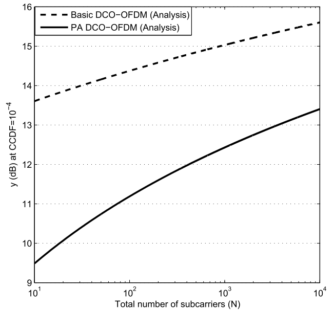
FIGURE 5. PAPR threshold values based on (40) to attain a CCDF of 10^{-4} against N for basic and PA DCO-OFDM signal with U = 5 , and P = 5 .
