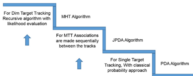
FIGURE 4. Comparative illustration for Probabilistic Data Association (PDA), Joint Probabilistic Data Association (JPDA) and Multiple-Hypothesis Tracking (MHT) Algorithm.
