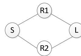
FIGURE 1. The basic coupling topology of a doublet.
