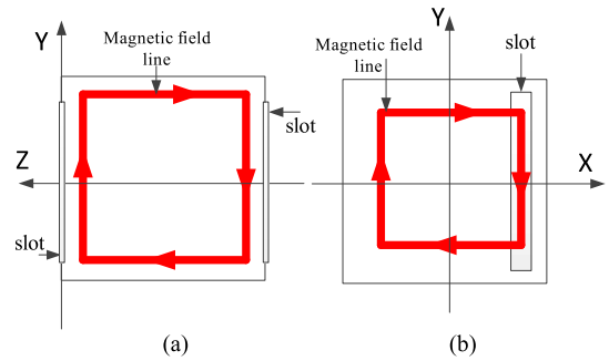
FIGURE 5. The magnetic field of Type-A filter (a) TE_{011} mode, (b) TM_{110} mode.
