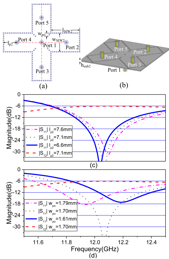
FIGURE 5. (a) Top view of the 1 to 4 SIW power divider, (b) 3D view, (c) Position of port 2 to 5 and (d) Width w_{po} effect on reflection coefficient of the 1 to 4 SIW power divider (The optimum dimensions are h_{sub2} = 0.508 mm, l_{p2} = 7.1 mm, w_{SIW2} = 9.9 mm, l_{SIW2} = 15.2 mm, w_{po} = 1.70 mm).
