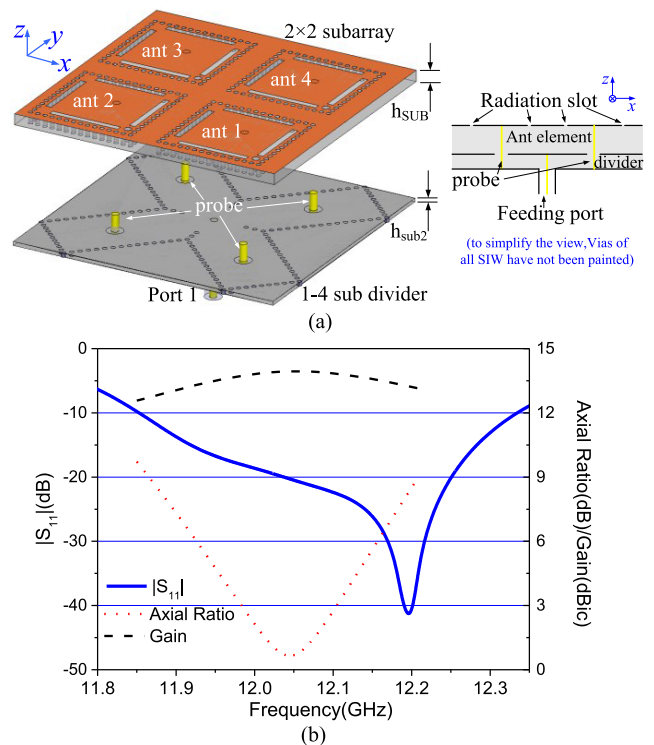
FIGURE 6. (a) 3D antenna assembly view, (b) The reflection coefficient, axial ratio and gain of the 2×2 CP SIW slot antenna subarray fed by the proposed 1 to 4 SIW power divider.
