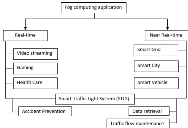
FIGURE 2. Proposed fog computing application taxonomy.
