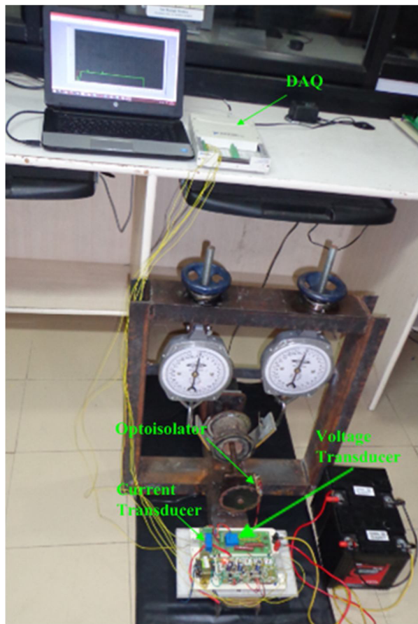
FIGURE 7. Experimental setup.
