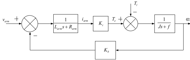
FIGURE 1. PMDC motor model.
