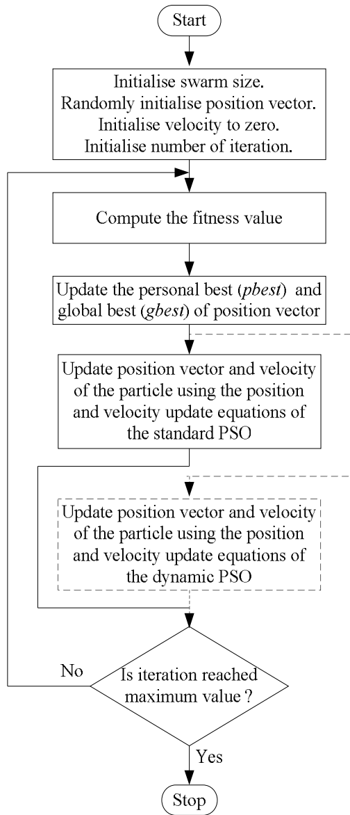
FIGURE 3. Flowchart of the standard as well as dynamic PSO algorithm.
