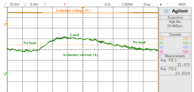
FIGURE 8. Instantaneous armature current and voltage waveforms.
