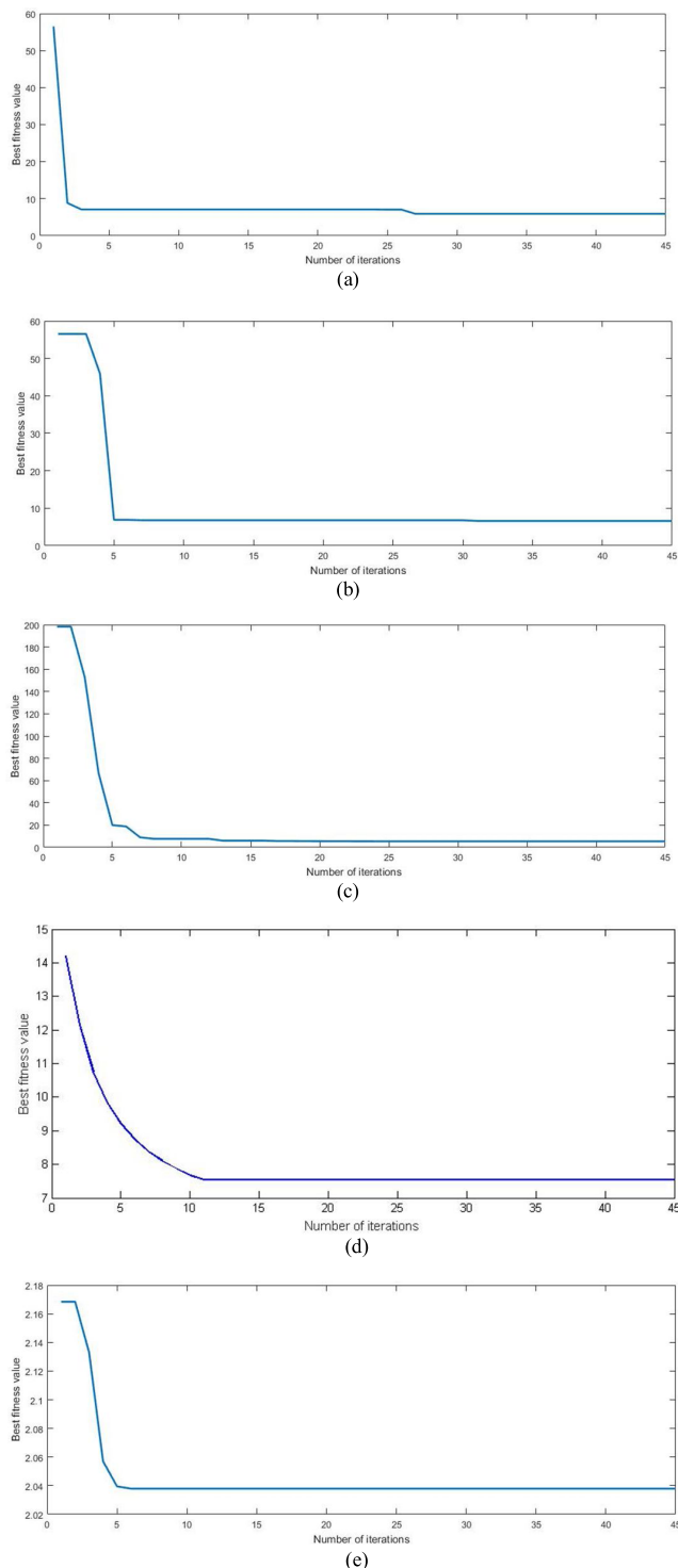
FIGURE 6. Best fitness value versus number of iterations. (a) Standard PSO algorithm. (b) Dynamic PSO with constant inertia weight algorithm. (c) Dynamic PSO with varying inertia weight algorithm. (d) Artificial bee colony algorithm. (e) Ant colony optimization algorithm.
