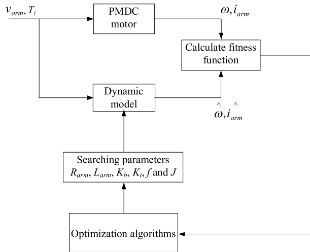
FIGURE 2. Estimation of PMDC motor parameters using optimization algorithm.
