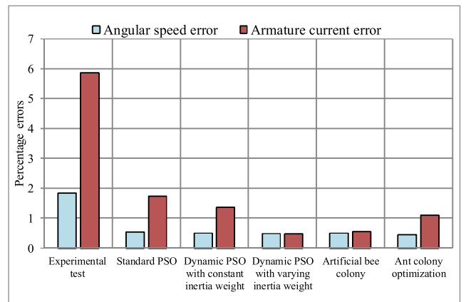
FIGURE 9. Percentage error of angular speed and armature current.
