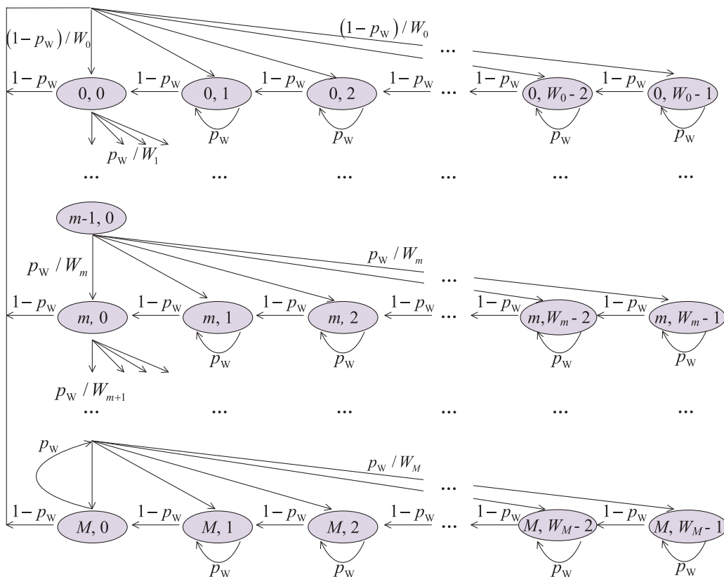
FIGURE 3. Markov model of a Wi-Fi STA with IEEE 802.11 DCF when coexisting with LTE-U network.
