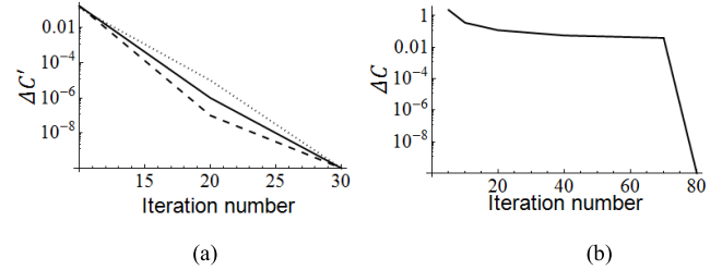
FIGURE 8. Cost functions associated with the extended coupling matrix from: (a) Table 6; and (b) Table 7. (solid line-Nelder Mead, Dashed-Simulated Annealing, dots-Differential Evolution).
