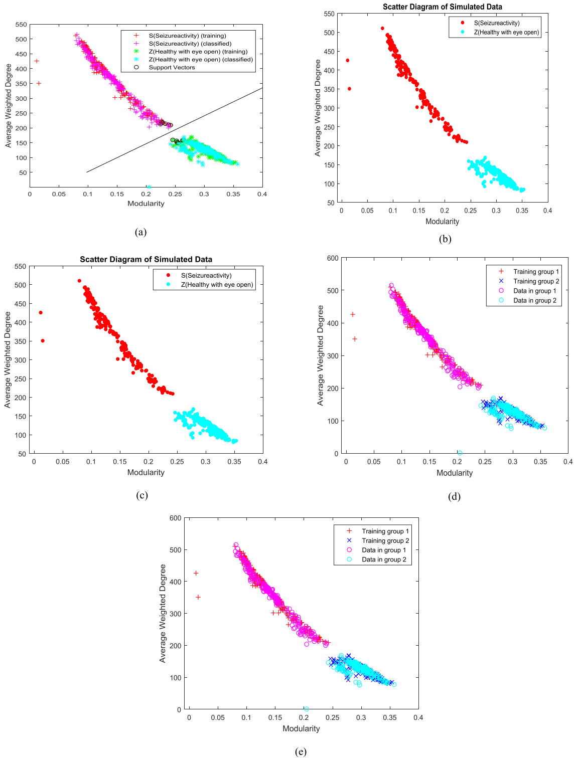
FIGURE 11. Illustration of classification accuracy for set A vs set E by combining two features and using classifier (a) SVM with linear kernel, (b) SVM with RBF kernel, (c) SVM classifier with polynomial, (d) KNN with K=3, (e) KNN with K=10.
